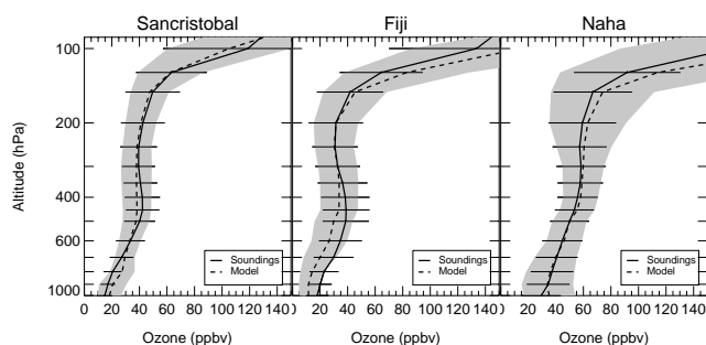
Fig. 3. Comparison of average vertical profiles for ozone as simulated by CAM-Chem for the last of a 10-yr run (dashed lines) with observations at three sites (San Cristobal, Galapagos, 1^\circ \text{S} – 89^\circ \text{W} ; Fiji, 18^\circ \text{S} – 178^\circ \text{E} ; Naha, Japan, 26^\circ \text{N} – 127^\circ \text{E} ) of the SHADOZ and WUOZC ozonesonde networks (solid lines). Shaded areas and horizontal bars represent the standard deviation of modelled fields and observations, respectively.
