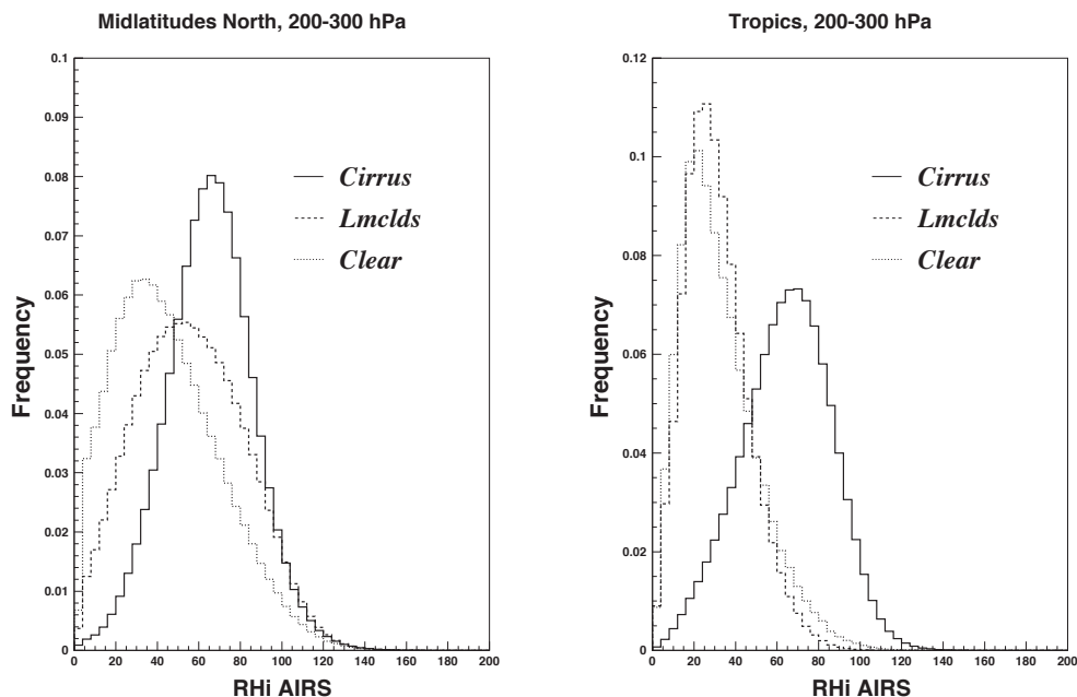
Fig. 3. Distributions of AIRS relative humidity RH_A for three classes of AIRS cloud properties in two latitude bands: Northern Hemisphere midlatitudes ( 40\text{--}60^\circ , left) and tropics ( 20^\circ\text{ N--}20^\circ\text{ S} , right). For lmclds and clear situations RH_A is all measurements in pressure layers 200–250 and 250–300 hPa. For cirrus situations RH_A is restricted to one of these two pressure layers enclosing the cloud pressure p_{\text{cld}} .
