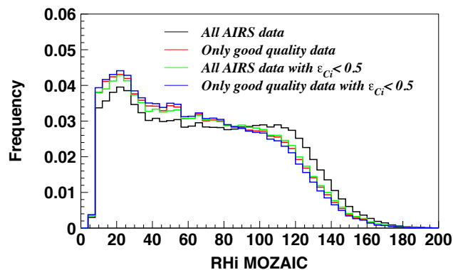
Fig. 1. Distributions of relative humidity seen from MOZAIC \text{RH}_i in collocation with AIRS data (all qualities combined) or only with good quality AIRS data for all cloud types and when removing the thickest cirrus clouds with \epsilon_{\text{cld}} > 0.5 .
