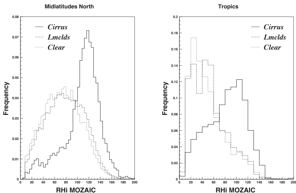
Fig. 4. Distributions of relative humidity seen by MOZAIC RH_M for three classes of AIRS cloud properties in two latitude bands: Northern Hemisphere midlatitudes ( 40\text{--}60^\circ , left) and tropics ( 20^\circ\text{ N--}20^\circ\text{ S} , right). For lmclds and clear situations RH_M is all measurements between 200 and 300 hPa, for cirrus situations measurements are taken at pressures close to the cloud pressure so that |p_M - p_{\text{cld}}| < 50 hPa. The binning for the tropics is less resolved due to the smaller sample size in the tropics.
