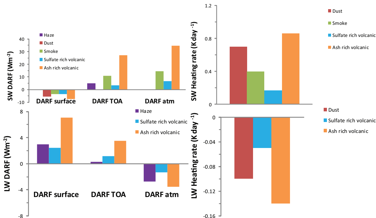
Fig. 15. (a) SW direct radiative forcings (DARFS) and (b) SW heating rates for haze (Quinn et al., 2007), dust (Stone et al., 2007), smoke (Stone et al., 2008), and ash rich and sulfate rich volcanic aerosols (this study). Values of forcing for dust were only available at the surface. (c) LW DARFs for haze (Ritter et al., 2005) and ash rich and sulfate rich volcanic aerosols (this study). (d) LW cooling rates for dust (Stone et al., 2007) and ash rich and sulfate rich volcanic aerosols (this study).
