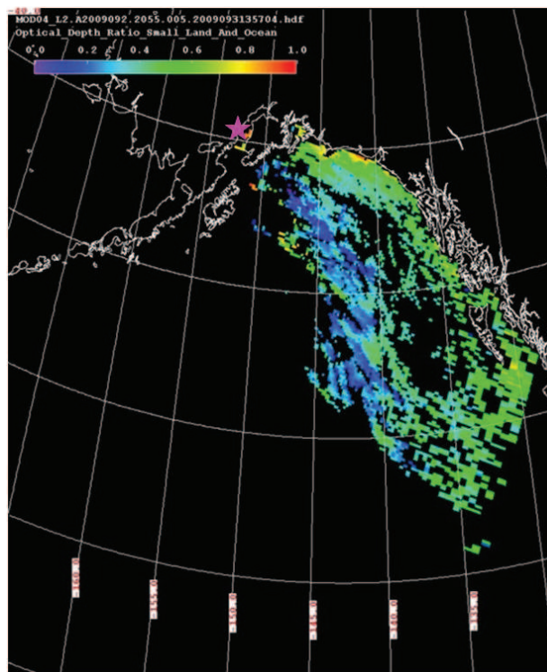
Fig. 5. Terra MODIS fine mode fraction AOD on 2 April at 20:55 UTC. Mt. Redoubt is marked by a star.
