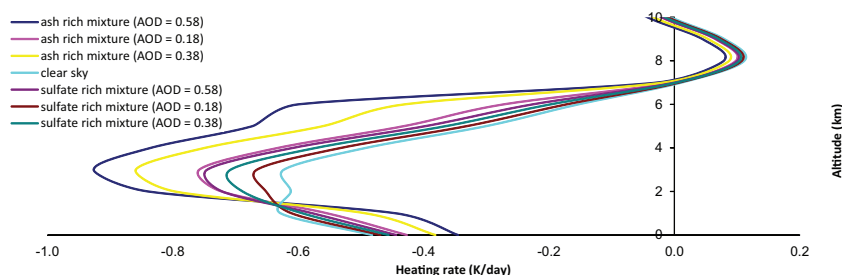
Fig. 10. The effect of aerosol composition and AOD(550 nm) of a thin plume ( \sim 2.5\text{--}7 km) on LW cooling rate.
