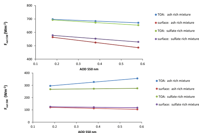
Fig. 7. The relationship between net SW flux and AOD(550 nm) at an AOD range of 0.18–0.58 for two aerosol mixtures at the TOA and surface over seawater (top panel) and snow (bottom panel). SZA is 55°. The R^2 regressions for all lines are greater than 0.99.
