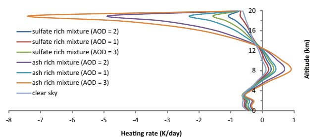
Fig. 14. The effect of aerosol composition and AOD(550 nm) of a thick plume (~3–20 km) on LW cooling rate.
