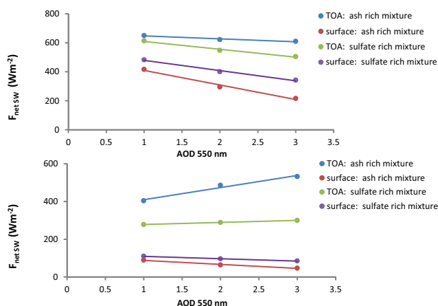
Fig. 11. The relationship between net SW flux and AOD(550 nm) at an AOD range of 1–3 for two aerosol mixtures at the TOA and surface over seawater (top panel) and snow (bottom panel). \text{SZA} = 55^\circ . The R^2 regressions for all lines are greater than 0.95.
