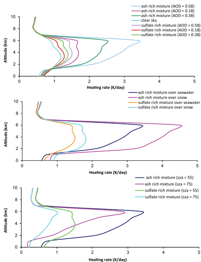
Fig. 8. (a) The effect of aerosol composition and AOD(550 nm) of a thin plume ( \sim 2.5\text{--}7 km) on SW heating rate. \text{SZA} = 55^\circ and surface type is seawater for all cases. (b) The effect of aerosol composition of a thin plume ( \sim 2.5\text{--}7 km) and surface type on SW heating rate. \text{SZA} = 55^\circ and AOD (550 nm) = 0.58 for all cases. (c) The effect of aerosol composition of a thin plume ( \sim 2.5\text{--}7 km) and solar zenith angle (SZA) on SW atmospheric heating rate. The AOD(550 nm) = 0.58 and the surface type is seawater for all cases.
