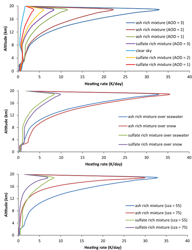
Fig. 12. (a) The effect of aerosol composition and AOD(550 nm) of a thick plume ( \sim 3 – 20 km) on SW heating rate. SZA = 55^\circ and surface type is seawater for all cases. (b) The effect of aerosol composition of a thick plume ( \sim 3 – 20 km) and surface type on SW heating rate. SZA = 55^\circ and AOD(550 nm) = 3 for all cases. (c) The effect of aerosol composition of a thick plume ( \sim 3 – 20 km) and solar zenith angle (SZA) on SW heating rate. The AOD(550 nm) = 3 and the surface type is seawater for all cases.
