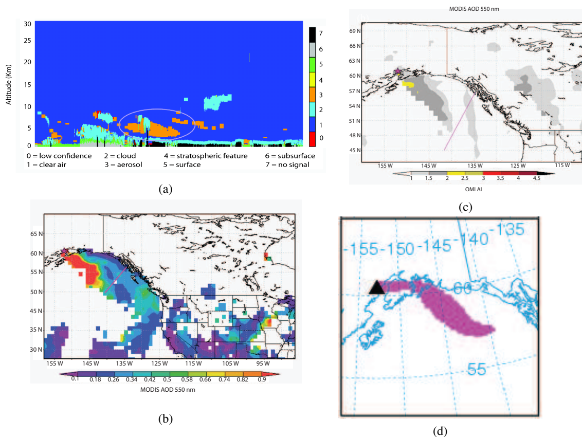
Fig. 4. (a) Vertical feature mask from CALIPSO between 11:31 UTC and 11:45 UTC on 2 April. The plume of interest is circled. (b) MODIS AOD(550 nm) daily mean for 2 April. Mt. Redoubt is marked with a star. CALIPSO path is shown with a line. (c) Same as (b), except for OMI AI. (d) Transport of ash plume (shown in pink) from the 2 April eruption as predicted by the HYSPLIT model. Eruption duration of 12 hours and an ash column height of 4.6 km were used.
