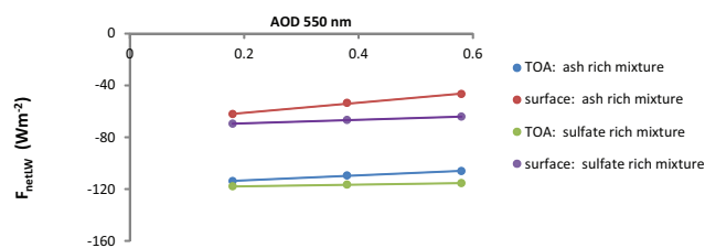
Fig. 9. The relationship between net LW flux and AOD(550 nm) at an AOD range of 0.18–0.58 for two aerosol mixtures at the TOA and surface. The R^2 regressions for all lines are greater than 0.99.
