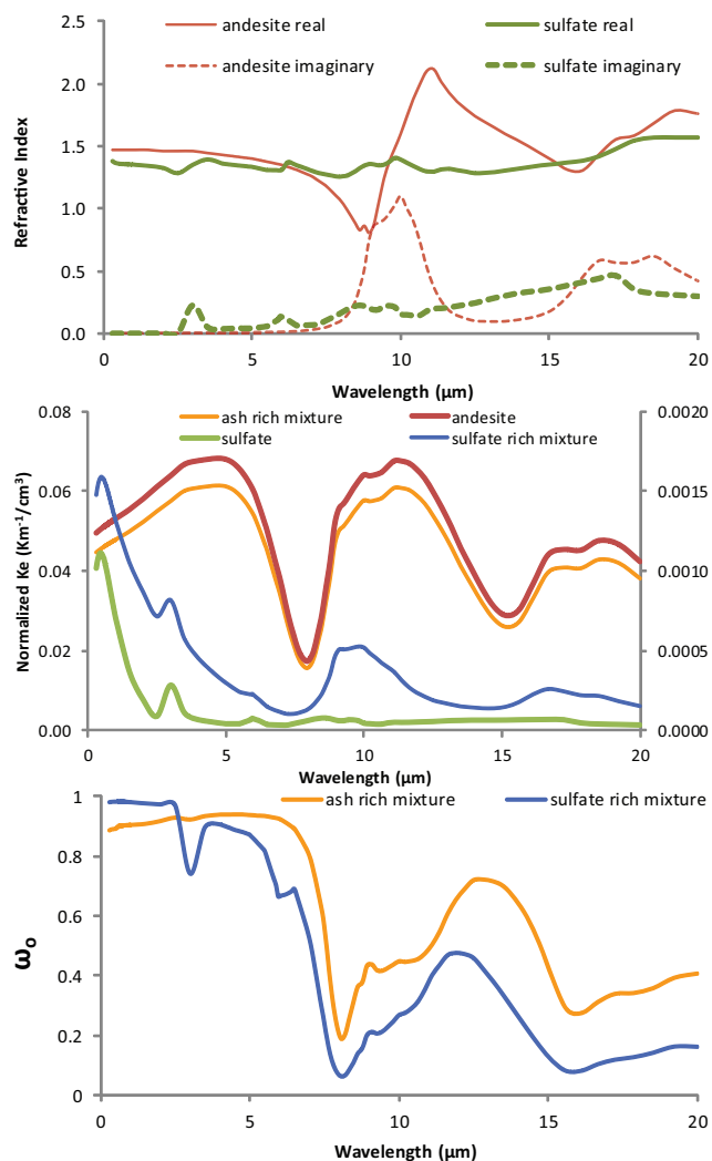
Fig. 1. (a) Spectral dependence of refractive indices of ash and sulfate. (b) Concentration normalized extinction coefficients ( K_e ) versus wavelength for an ash rich mixture containing an ash to sulfate ratio of 9 to 1 and an effective radius for ash R_{\text{eff}} = 5 \mu\text{m} compared to andesite with R_{\text{eff}} = 5 \mu\text{m} (right axis) and for a sulfate rich mixture containing an ash to sulfate ratio of 1 to 9 and an effective radius for ash R_{\text{eff}} = 1.5 \mu\text{m} compared to sulfate with R_{\text{eff}} = 0.5 \mu\text{m} (left axis). (c) Single scattering albedo ( \omega_0 ) versus wavelength for an ash rich mixture containing an ash to sulfate ratio of 9 to 1 and R_{\text{eff}} = 5 \mu\text{m} and a sulfate rich mixture containing an ash to sulfate ratio of 1 to 9 and R_{\text{eff}} = 1.5 \mu\text{m} .
