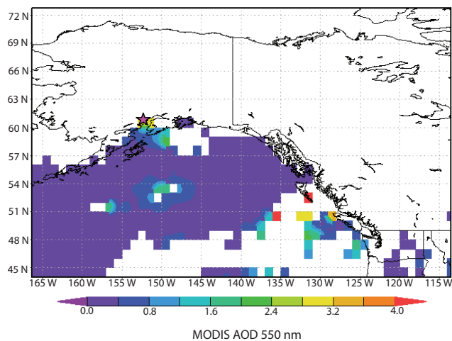
Fig. 6. MODIS AOD(550 nm) daily average for 27 March. These AOD values were the highest over the entire course of the explosive eruptions, due to aerosol produced by the very powerful eruption at 17:24 UTC on March 26 and the eruptions that followed on 27 March.
