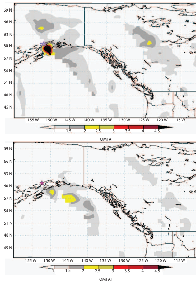
Fig. 3. OMI AI for (a) 26 March and (b) 4 April. The location of Mt. Redoubt is marked by a star.
