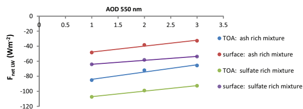
Fig. 13. The relationship between net LW flux and AOD(550 nm) at an AOD range of 1–3 for two aerosol mixtures at the TOA and surface. The R^2 regressions for all lines are greater than 0.96.
