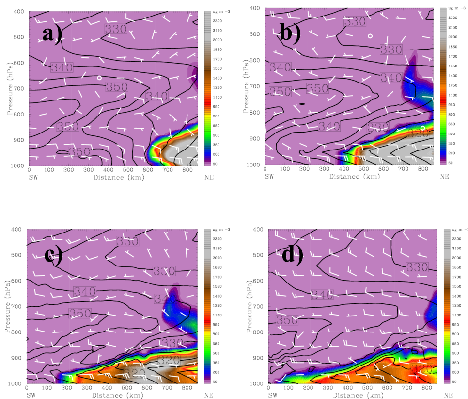
Fig. 10. The cross-section distribution of wind field, theta-e (contour) and \text{PM}_{10} concentration (colored) along NE1 in Fig. 9 at (a) 18:00 UTC, 20 March (b) 00:00 UTC, 21 March (c) 06:00 UTC, 21 March (d) 12:00 UTC, 21 March. A full (half) wind barb indicates 5 \text{ m s}^{-1} ( 2.5 \text{ m s}^{-1} ).
