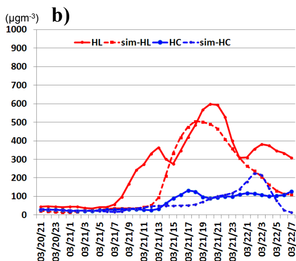
Fig. 8. Temporal variation of observation (solid) and simulation (dashed) \text{PM}_{10} concentration around Taiwan at stations, SL, CH, MG, HL and HC from 21:00 LST, 20 March to 07:00 LST, 22 March 2010.
