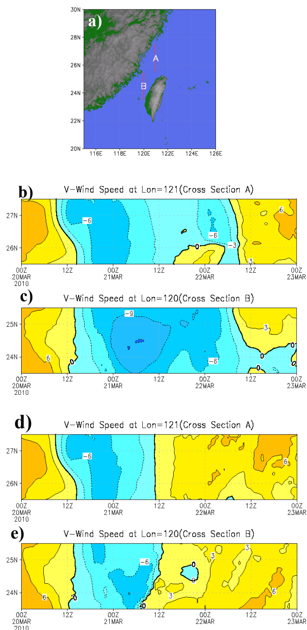
Fig. 14. (a) Schematic illustration of cross-sections A and B. (b) Temporal variation of N-S component of wind speed during 20–23 March 2010 for control run along cross A. The contour is shown in 3 \text{ m s}^{-1} interval. (c) Same as (b) but for along cross B. (d) Same as (b) but for Case QT along cross A. (e) Same as (b) but for case QT along cross B.
