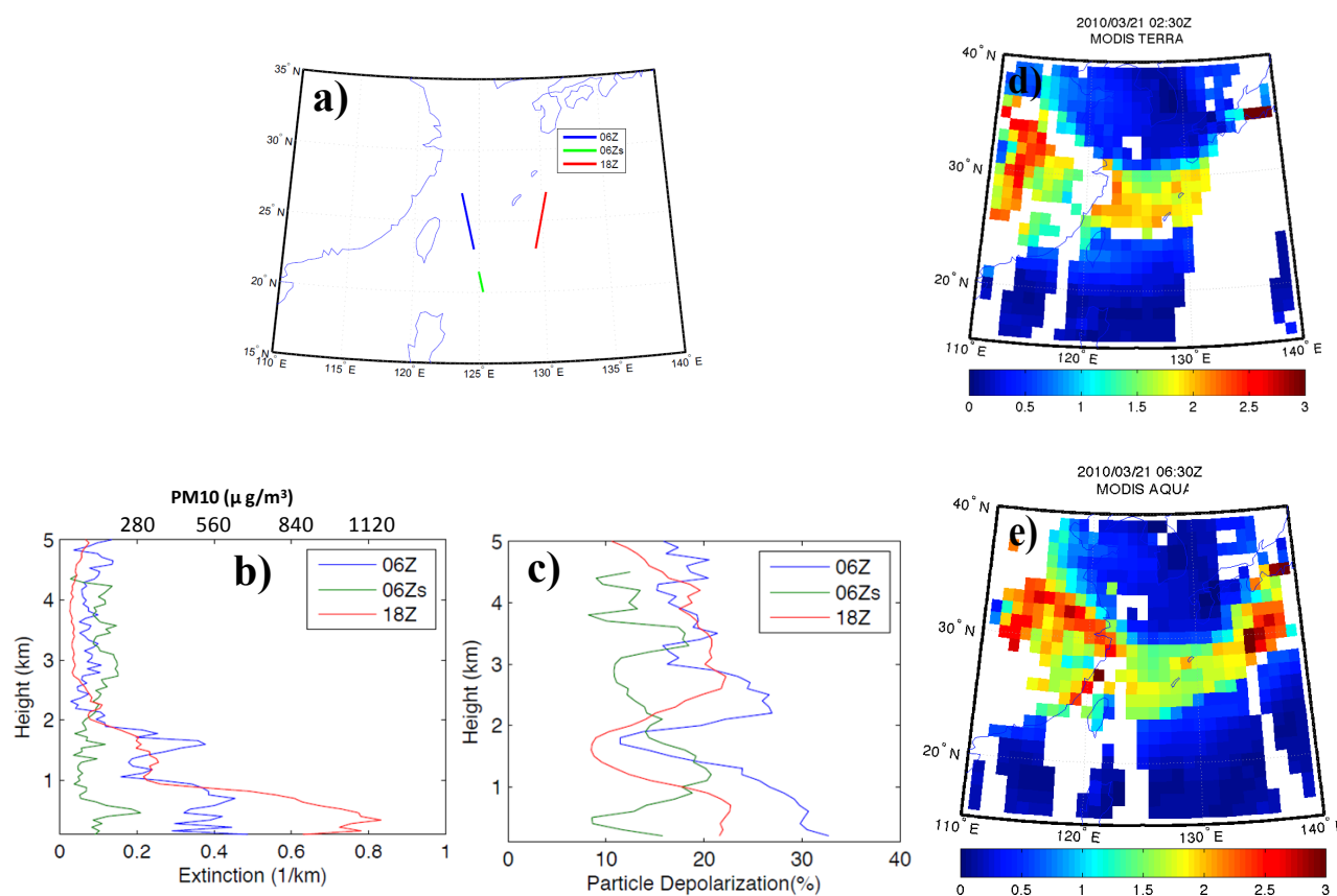
Fig. 6. (a) The CALIPSO orbit tracks around Taiwan at 06:00 UTC (blue and green), and 18:00 UTC (red), 21 March 2010. (b) The vertical distribution of extinction coefficient and PM 10 concentration deduced from CALIPSO Lidar at orbit tracks in (a) around Taiwan. (c) The vertical distribution of the percentage of depolarization ratio from CALIPSO Lidar at orbit tracks in (a) around Taiwan. (d) The aerosol optical depth (AOD) deduced from the MODIS satellite at 02:30 UTC, 21 March 2010. (e) Same as (d) but for at 06:30 UTC.
