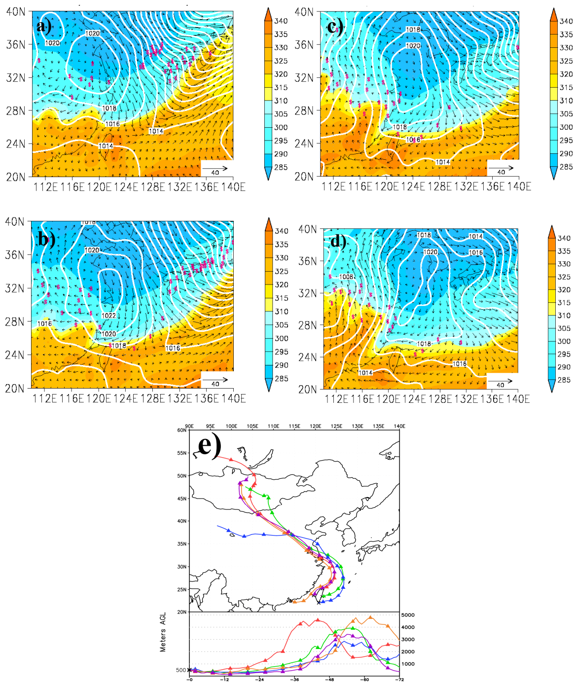
Fig. 4. (a) The ground dust reports (denoted by dollar signs) are from Global Telecommunication System (GTS) data. Wind field and theta-e (colored) are deduced from NCEP GFS data at 925 hPa level and contour lines are represented for sea-surface pressure at 18:00 UTC 20 March 2010. (b) Same as (a) but for 00:00 UTC, 21 March 2010. (c) Same as (a) but for 06:00 UTC, 21 March 2010. (d) Same as (a) but for 12:00 UTC, 21 March 2010. (e) Result of the HYSPLIT model 3-day backward trajectory analysis at altitude of 500 m starting from the time of peak value for stations at Taiwan (WL, HL, HC, MG) and TM at Hong Kong.
