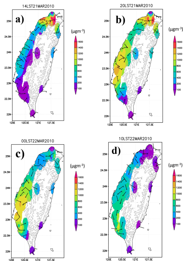
Fig. 3. Spatial distribution of observation PM 10 (μg m -3 ) concentration and wind recorded in Taiwan at (a) 14:00 LST, 21 March (b) 20:00 LST, 21 March (c) 00:00 LST, 22 March (d) 10:00 LST, 22 March.
