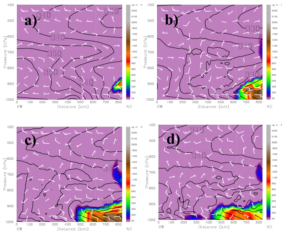
Fig. 11. The cross-section distribution of wind field, theta-e (contour) and \text{PM}_{10} concentration (colored) along NE2 in Fig. 9 at (a) 18:00 UTC, 20 March (b) 00:00 UTC, 21 March (c) 06:00 UTC, 21 March (d) 12:00 UTC, 21 March. A full (half) wind barb indicates 5 \text{ m s}^{-1} ( 2.5 \text{ m s}^{-1} ).
