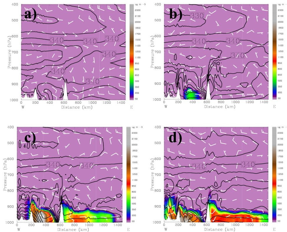
Fig. 13. The cross-section distribution of wind field, theta-e (contour) and PM 10 concentration along EW2 in Fig. 9 at (a) 18:00 UTC, 20 March (b) 00:00 UTC, 21 March (c) 06:00 UTC, 21 March (d) 12:00 UTC, 21 March. A full (half) wind barb indicates 5 m s -1 (2.5 m s -1 ).
