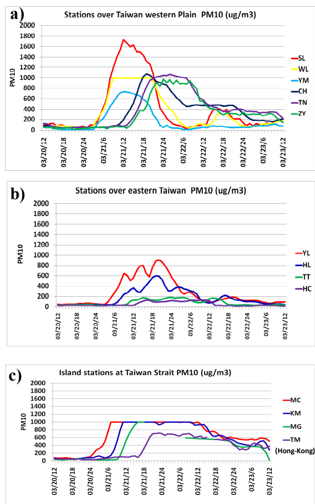
Fig. 2. (a) Hourly concentration variation of PM 10 (μg m -3 ) for the selected stations (SL, WL, YM, CH, TN and ZY) at Taiwan's western plain during 12:00 LST, 20–23 March 2010. (b) Hourly concentration variation of PM 10 (μg m -3 ) for the selected stations (YL, HL, TT and HC) at eastern Taiwan during 12:00 LST, 20–23 March 2010. (c) Hourly concentration variation of PM 10 (μg m -3 ) for the island stations (MC, KM and MG) in the Taiwan Strait and station TM at Hong Kong during 12:00 LST, 20–23 March 2010.
