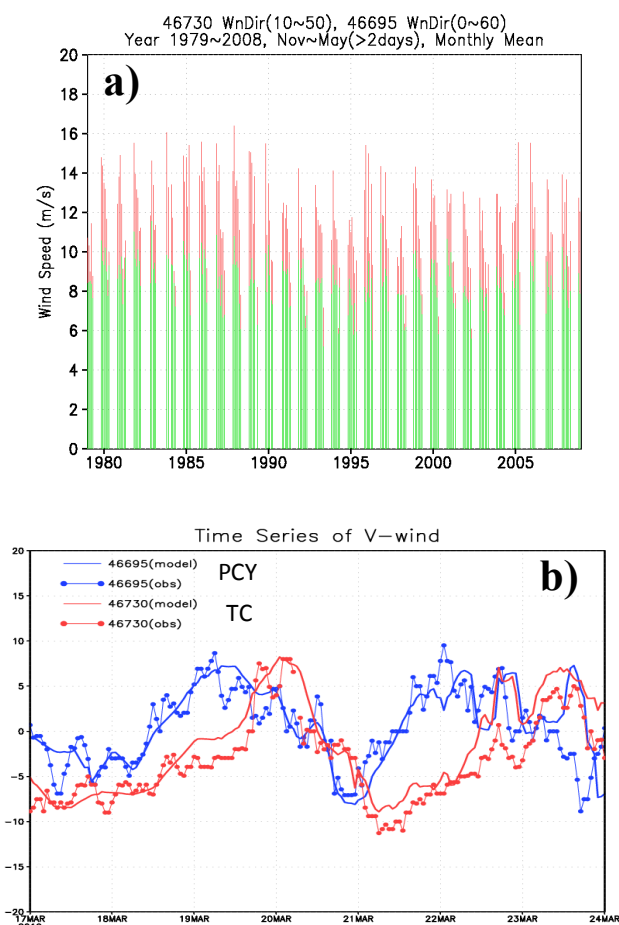
Fig. 5. (a) Time series of monthly average wind speed during northeasterly monsoon (November–May) for station TC (red bars) and station PCY (green bars) between 1979 and 2008. (b) The observation and simulation N–S component of wind speed at stations PCY (blue) and TC (red) during 00:00 LST, 17–24 March 2010.
