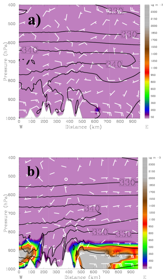
Fig. 12. The cross-section distribution of wind field, theta-e (contour) and \text{PM}_{10} concentration (colored) along EW1 in Fig. 9 at (a) 14:00 UTC, 20 March (b) 20:00 UTC, 20 March. A full (half) wind barb indicates 5 \text{ m s}^{-1} ( 2.5 \text{ m s}^{-1} ).
