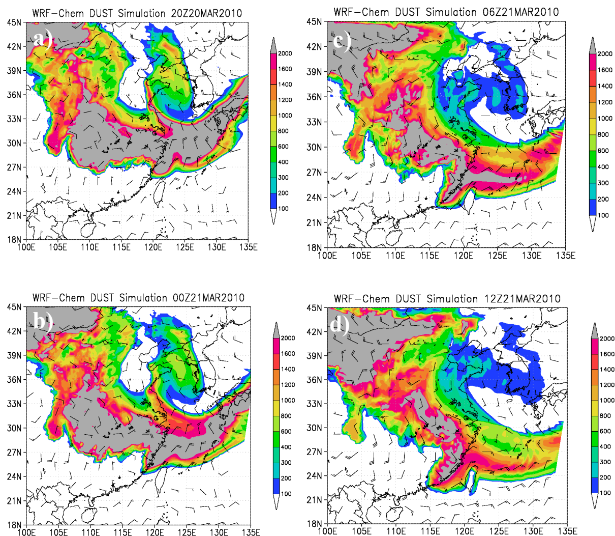
Fig. 7. The simulation spatial distribution of \text{PM}_{10} concentration and wind field at 1000 hPa. A full (half) wind barb indicates 5 \text{ m s}^{-1} ( 2.5 \text{ m s}^{-1} ). (a) 20:00 UTC, 20 March 2010. (b) 00:00 UTC, 21 March 2010. (c) 06:00 UTC, 21 March 2010. (d) 12:00 UTC, 21 March 2010.
