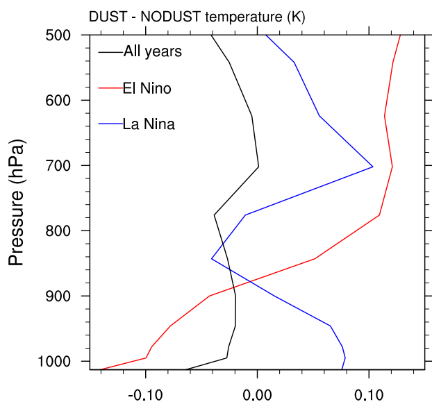
Fig. 15. As Fig. 14, but showing profiles of dust-induced temperature changes (difference between the DUST and NODUST runs). The dust-induced SST change is plotted at 1013 hPa.
