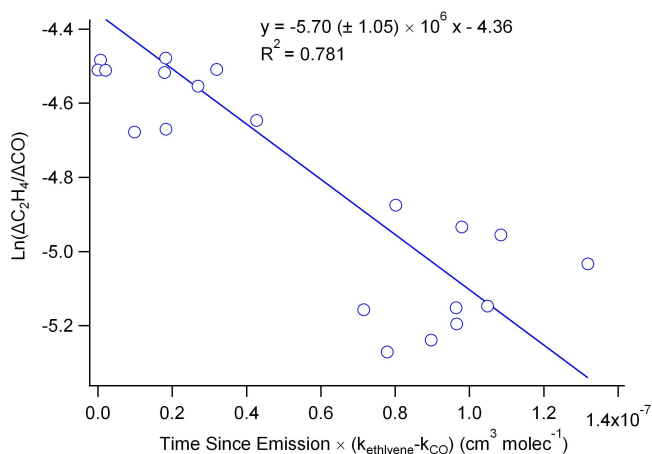
Fig. 6. \text{Ln}(\Delta\text{ethylene}/\Delta\text{CO}) vs. time since emission (h) \times (k_{\text{ethylene}} - k_{\text{CO}}) . Average OH in the plume from \sim 10:30 – 15:16 LT is initially estimated from the absolute value of the slope ( 5.70 \pm 1.05 \times 10^6 \text{ molec cm}^{-3} ) and then corrected for \text{O}_3 oxidation (see Sect. 3.2.2).
