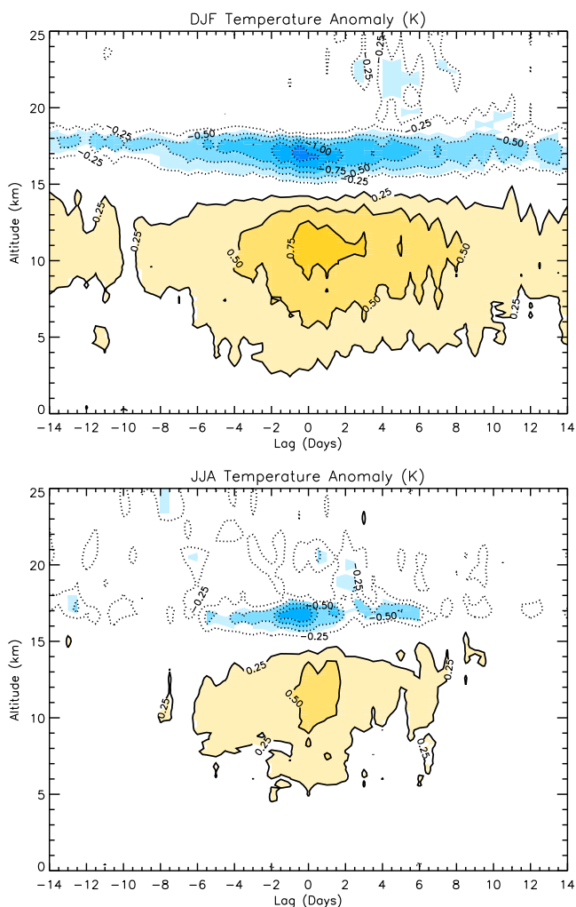
Fig. 8. Temperature anomaly within 1000 km of a deep convective cloud with cloud top greater than 17 km, contoured as a function of time and altitude during (top) DJF and (bottom) JJA. The contour interval is 0.25 K, and anomalies that exceed the 99 % significance level appear in color. Orange and red colors correspond to positive anomalies, blue colors correspond to negative anomalies.
