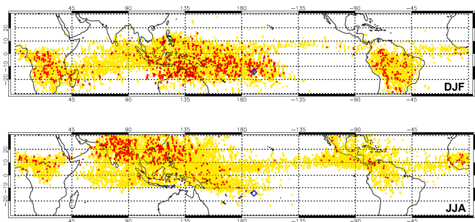
Fig. 2. Spatial distribution of deep convective cloud top pixels greater than 15 km (yellow) and greater than 17 km (red) during DJF (top) and JJA (bottom). The location of the SHADOZ station American Samoa is marked with a blue diamond.
