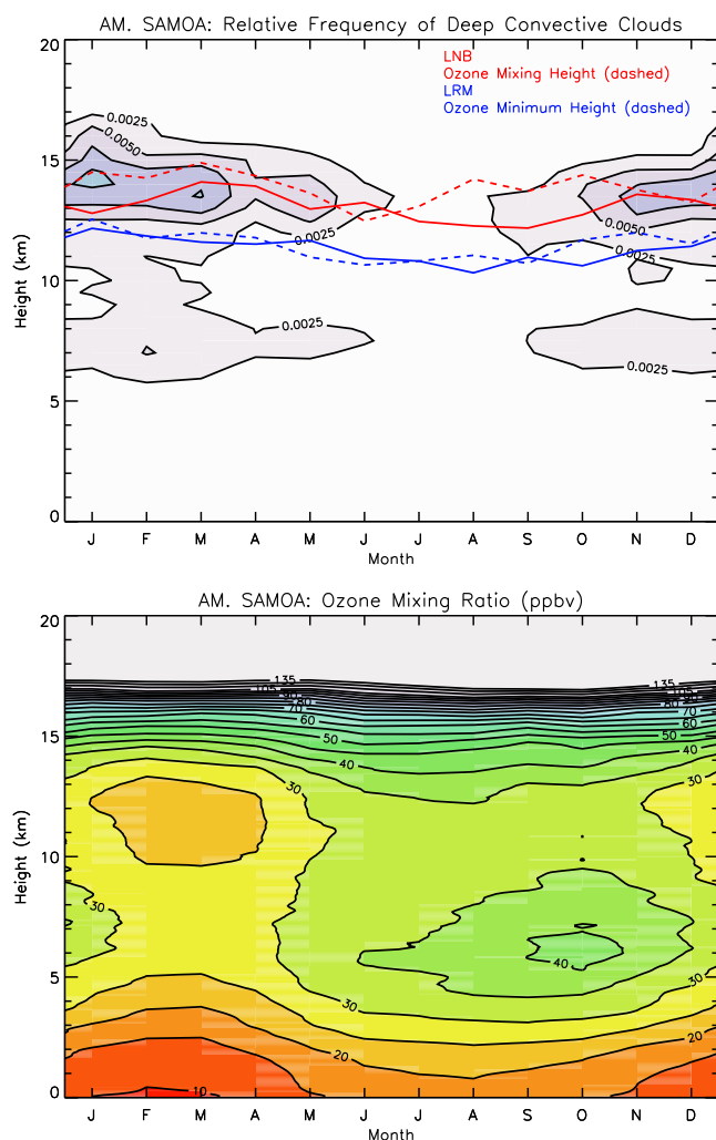
Fig. 9. (Top) annual cycle of the relative frequency distribution of deep convective cloud top heights within 1000 km of American Samoa (contours). Also included is the annual cycle of the LNB (red, solid), the ozone mixing height (red, dashed), the LRM height (blue, solid), and the ozone minimum height (blue, dashed). (Bottom) annual cycle of the ozone concentration (ppbv) at American Samoa, similar to Fig. 3d in Thompson et al. (2011). Orange and red colors indicate relatively low values, blue colors indicate relatively high values.
