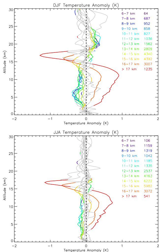
Fig. 6. Average temperature anomaly profiles for GPS soundings within \pm 6 \text{ h} and 1000 km of a maximum deep convective cloud greater than 17 km (red), between 16–17 km (orange), between 15–16 km (yellow), and so on, during (top) DJF and (bottom) JJA. Anomalies that exceed the 99 % significance level appear in color. The number of profiles that go into each anomaly profile is given on the right side of the figure.
