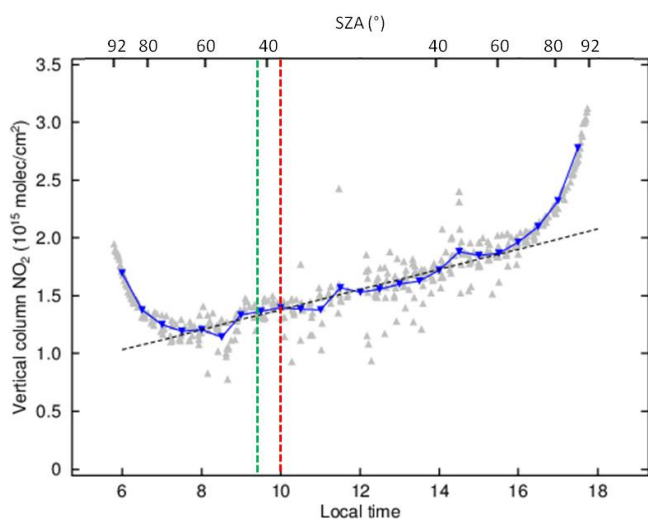
Fig. 5. Diurnal cycle of stratospheric NO 2 vertical columns on 15 October 2009 (grey: single measurements, blue: data binned to 0.5 h resolution). The black dashed line is the derived daytime linear increase, the green dashed line gives the approximate GOME-2 overpass time and the red line the SCIAMACHY overpass.
