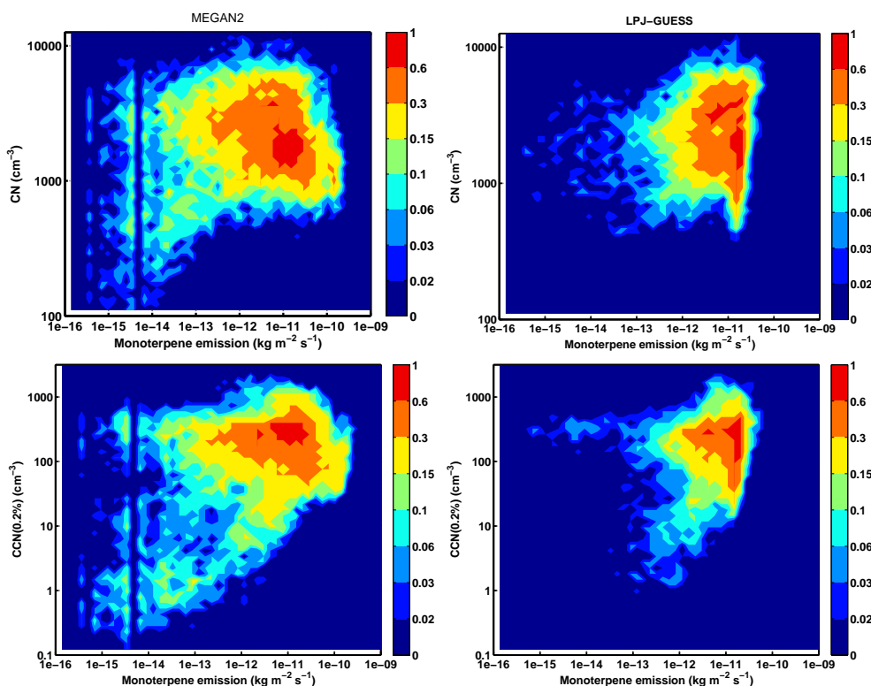
Fig. 6. 2-D histograms (density plots) of the monoterpane emission (x-axis) versus CN concentration (upper panels) and CCN(0.2%) concentration (lower panels) from ORGSULACT simulations. The histograms are calculated from monthly averages for each model grid box over land surface and the maximum value is scaled to unity. Surface level aerosol number concentrations are calculated from 5 yr of model simulation.
