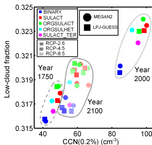
Fig. 11. Global average CCN(0.2 %) ( \text{cm}^{-3} ) versus global average low-cloud fraction from all simulations and time periods. Grey lines are drawn to show the separation of the years 1750, 2000 and 2100.
