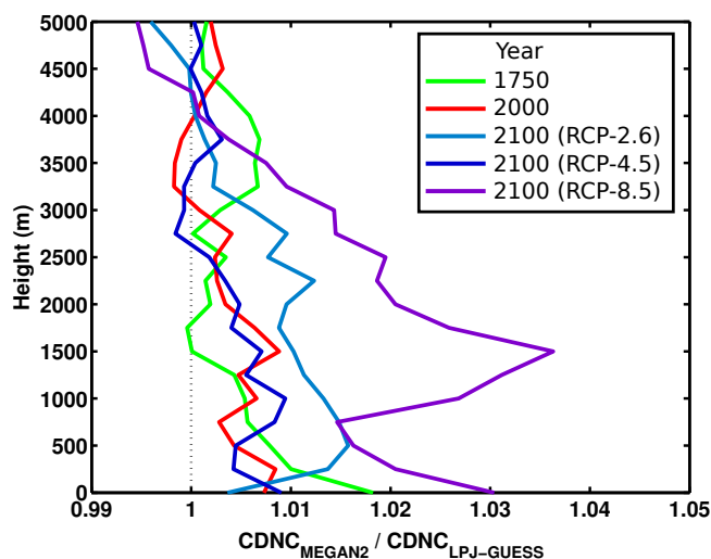
Fig. 9. Vertical profiles of global average CDNC ratio with BVOC emissions from MEGAN2 and LPJ-GUESS, calculated as \text{CDNC}_{\text{MEGAN2}}/\text{CDNC}_{\text{LPJ-GUESS}} . Results are averaged over the SULACT and ORGSULACT experiments.
