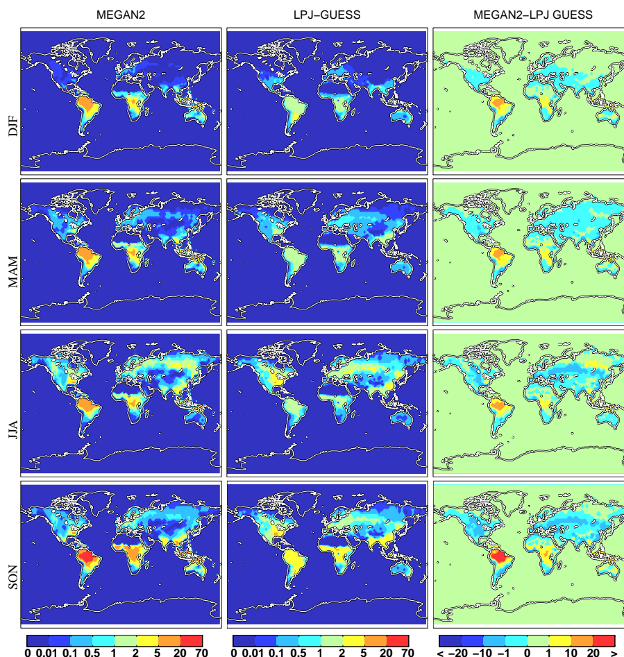
Fig. 1. Monoterpane emission fields from MEGAN2 and LPJ-GUESS models for different seasons ( 10^{-11} \text{ kg m}^{-2} \text{ s}^{-1} ) in the year 2000. Also shown is the difference of the two models.
