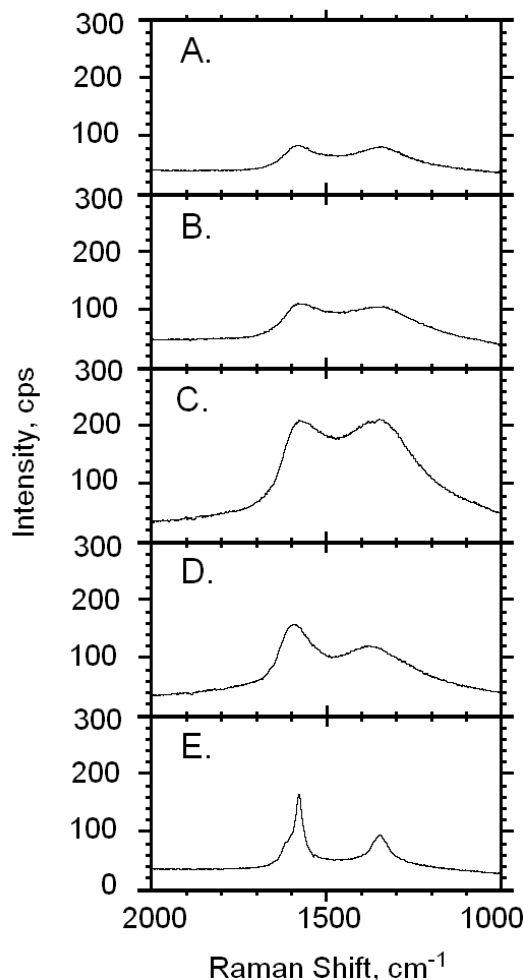
Fig. 8. Raman spectra of reference materials including soot generated by burning propane gas in our laboratory (A), Fluka humic acid (B), Pahokee peat humic acid (C), Leonardite humic acids (D), and graphite (E) are shown.
