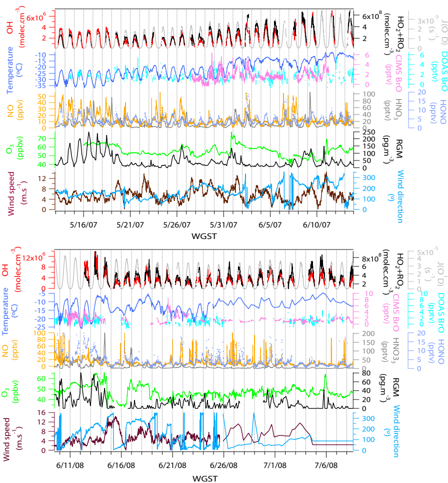
Fig. 2. Time series of measurements of HO 2 + RO 2 , OH, J(\text{O}^1\text{D}) , BrO, temperature, NO, HNO 3 , HONO, O 3 , RGM, wind speeds and directions on a 10 min time base in spring 2007 (top panel) and summer 2008 (bottom panel) Summit campaign.
