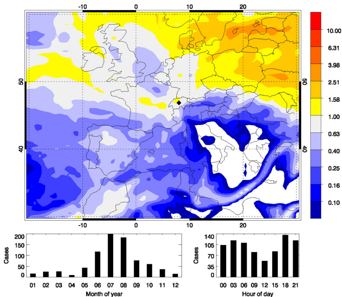
Fig. 13. Relative footprint map corresponding to low \text{CO}_2 but high APO and \text{O}_2 (subset 4). See Fig. 10 for further details
