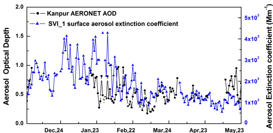
Fig. 2. Comparison of surface aerosol extinction coefficient at Surya village (SVL_1) with the column AOD measured by AERONET at neighboring urban center, Kanpur.
