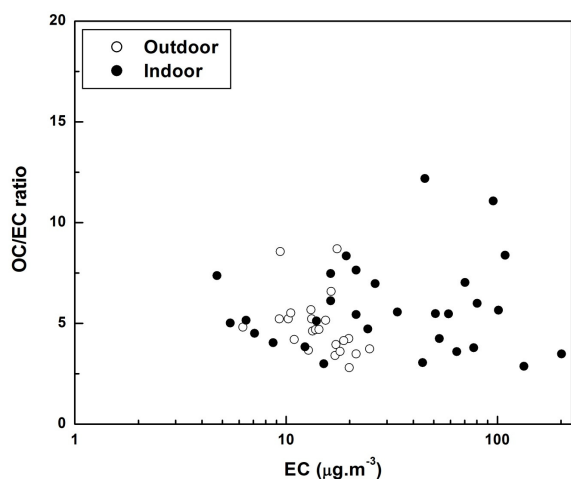
Fig. 7. Comparison between OC/EC ratio vs. EC concentration for indoor (SVI.1 village kitchen) and outdoor (SVI.1 village center) samples.
