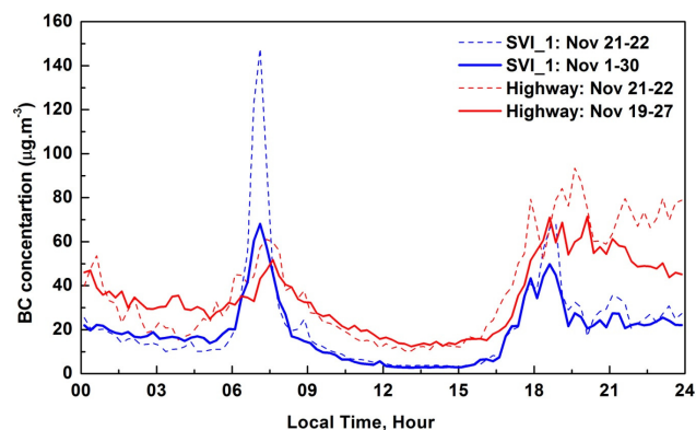
Fig. 5. Comparison of diurnal variation of BC concentration at Surya village (SVL1) center with highway measurement (locates around 3 km to the southeast of SVL1).
