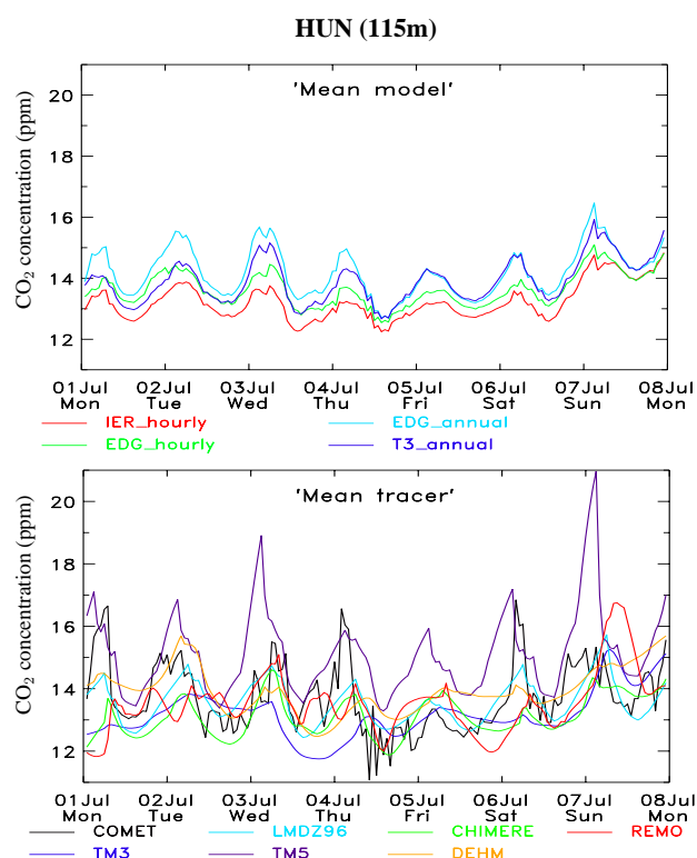
Fig. 4. Hourly simulated concentrations at HUN for 1 week in July: top: mean across all transport models for each emission inventory; bottom: mean across all emission inventory for each transport model.
