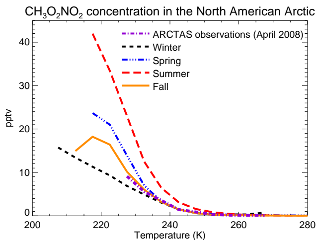
Fig. 3. Temperature binned mean values of the GEOS-Chem modeled \text{CH}_3\text{O}_2\text{NO}_2 24 h average concentrations over the North American Arctic for each season.
