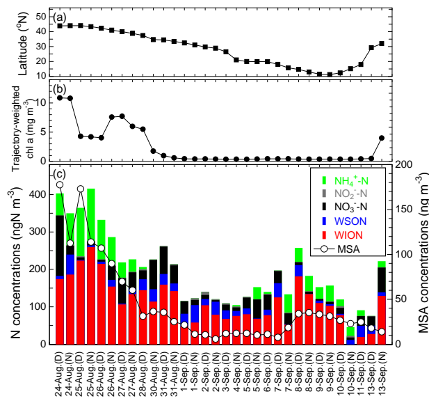
Fig. 3. Time series of (a) the average latitudinal location of the ship, (b) concentrations of trajectory-weighted chlorophyll- a and (c) fractions of organic (WSON and WION) and inorganic nitrogen together with concentrations of MSA. “D” means data obtained in daytime, whereas “N” means data obtained in nighttime.
