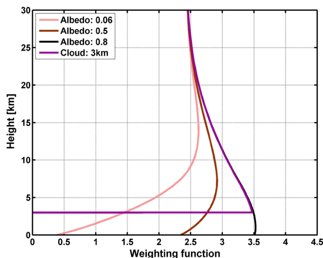
Fig. 4. Satellite weighting functions at 345.5 nm as function of surface albedo (0.06, 0.5 and 0.8 for a surface at sea level) and for a fully cloudy scene (cloud top height: 3 km, cloud albedo: 0.8). Calculations are made for a pure nadir observation geometry (line-of-sight angle: 0°) and a solar zenith angle of 45°.
