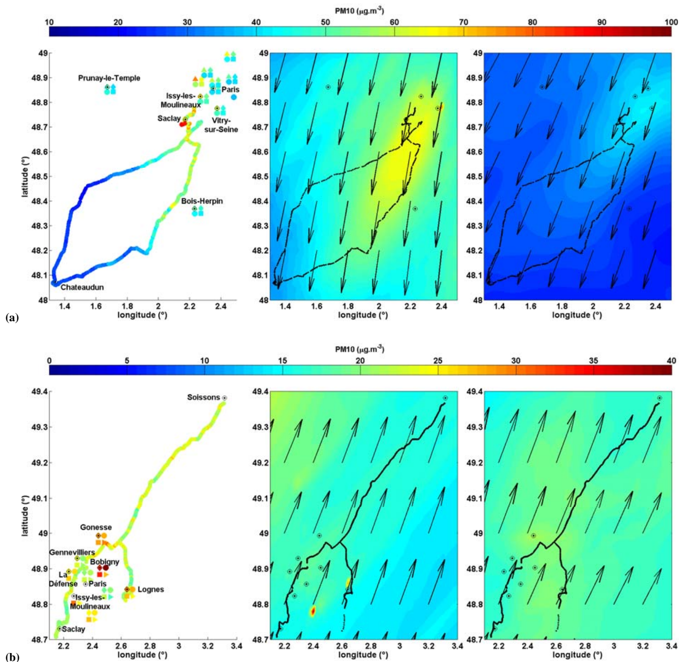
Fig. 3. Spatial distributions of wet PM 10 at 12:00 UT on 1 (a) and 15 (b) July derived from lidar measurements with the peri-urban relationship at 210 m height (left column) and simulated at 12:00 UT with the POLYPHEMUS model at 210 m height (central column) and the CHIMERE model at 250 m height (right column). Black arrows representing the wind at ~250 m height used in POLYPHEMUS and CHIMERE simulations are shown on the central and right panels. Dry PM 10 from AIRPARIF ground-based network are indicated by filled symbols at 13:00 (up triangles), 14:00 (diamonds), 15:00 (rounds), 16:00 (squares), 17:00 (right triangles), 18:00 LT (pentagrams) in the left column. Note that for 15 July a mixing of dust and peri-urban relationships has been used in lidar inversion.
