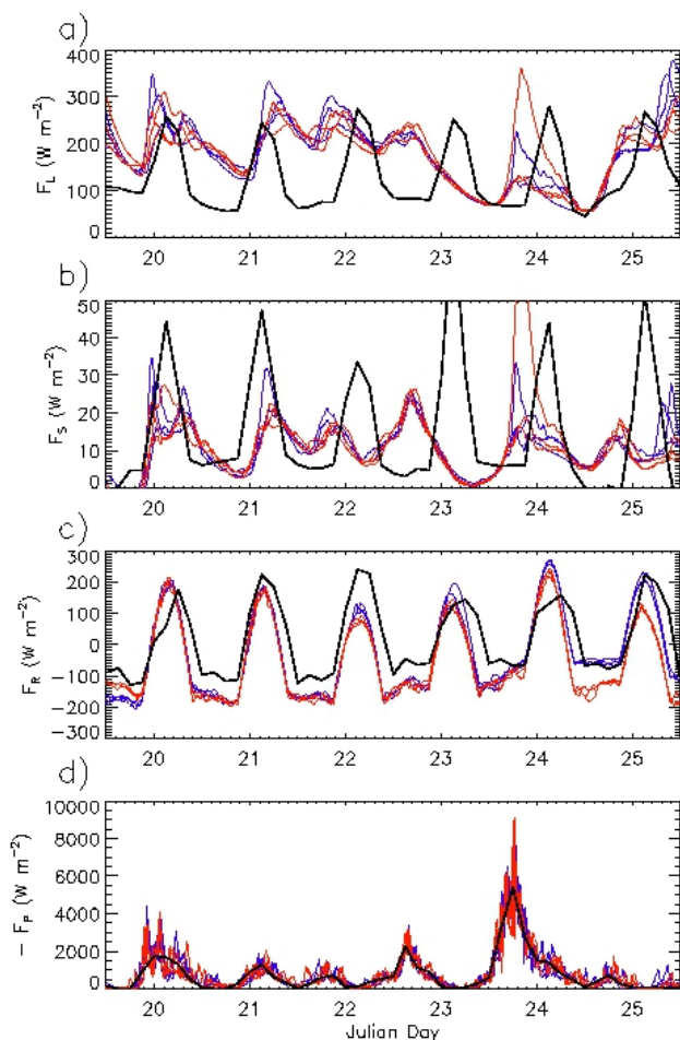
Fig. 5. As in Fig. 2, except timeseries of horizontally-averaged (a) surface latent heat flux, F_L , (b) surface sensible heat flux, F_S , (c) atmospheric radiative flux convergence, F_R , and (d) surface precipitation, F_P . Observed values are indicated by black lines.
