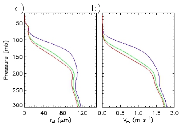
Fig. 16. Vertical profiles of ensemble- and horizontally-averaged mass-weighted (a) ice effective radius, r_{ei} , and (b) ice particle fallspeed, V_m , for PRIS (blue), POLL (green), and SPOLL (red). Presented results are averaged between 12:00 UTC 19 January and 12:00 UTC 25 January.
