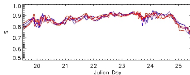
Fig. 7. As in Fig. 2, except for timeseries of the horizontally-averaged column saturation fraction.
