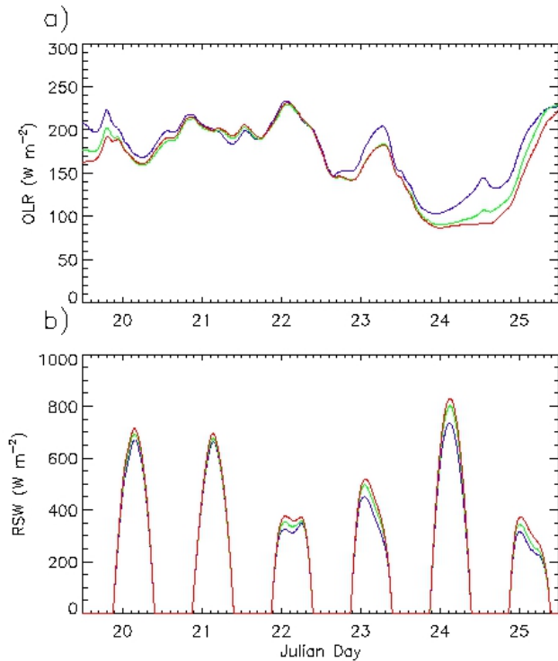
Fig. 12. Timeseries of ensemble- and horizontally-averaged TOA (a) outgoing longwave radiation (OLR) and (b) reflected shortwave radiation (RSW), for PRIS (blue), POLL (green), and SPOLL (red).
