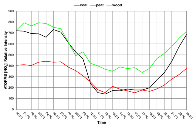
Fig. 9. Hourly averaged signal for nitrate for the Coal, Peat and Wood ATOFMS classes for the 4 low wind speed events (11–12 August 2008, 13–15 August 2008 and 22–23 August 2008).
