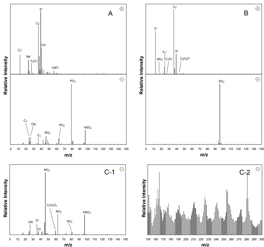
Fig. 13. Average dual ion mass spectra of ATOFMS particle classes; (A) EC-oil, (B) ECOC, and average negative ion mass spectra for (C-1) Oligomer ( m/z 0–150) and (C-2) Oligomer ( m/z 150–300).
