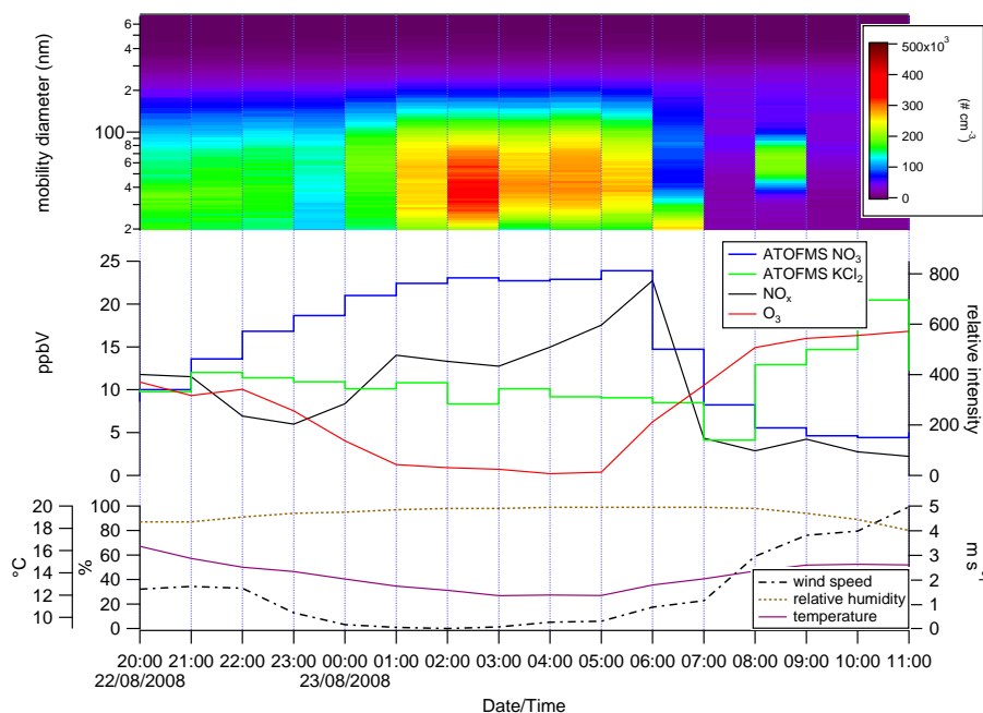
Fig. 8. Top panel: hourly integrated size resolved SMPS particle counts. Middle panel: hourly averaged ATOFMS signal for [\text{NO}_3]^- and [\text{KCl}_2]^+ , hourly averaged mixing ratios for \text{NO}_x and \text{O}_3 . Bottom panel: hourly averaged wind speed, relative humidity and temperature.
