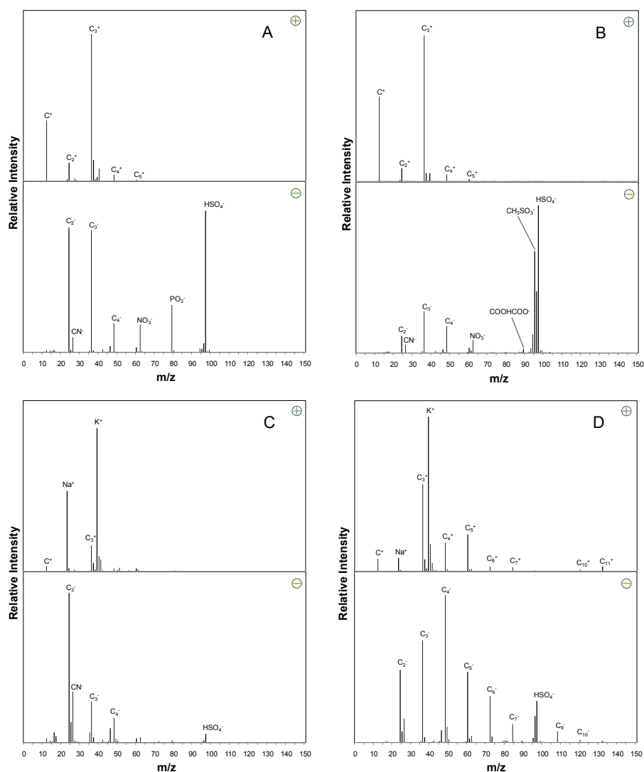
Fig. 12. Average dual ion mass spectra of ATOFMS particle classes; (A) EC-phos, (B) EC-MSA, (C) EC-domestic (D) EC-background.
