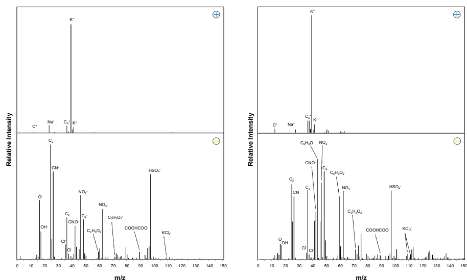
Fig. 5. Average dual ion mass spectra of ambient particles classified as “Wood” (left) and particles sampled during the wood combustion experiment (right).
