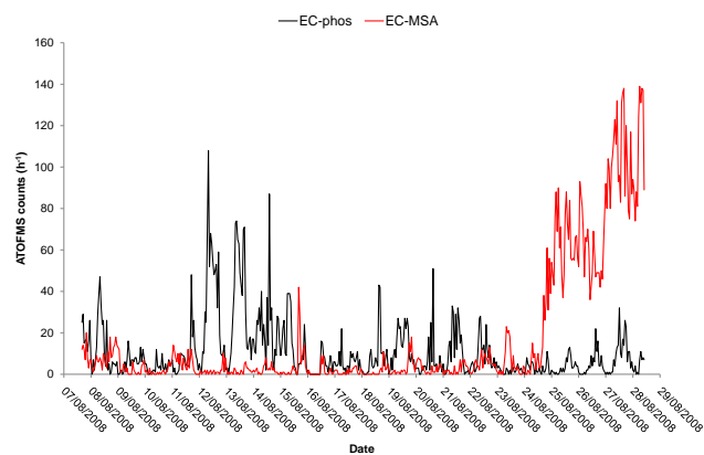
Fig. 14. Hourly integrated particle counts for EC-phos and EC-MSA particles for 7–28 August 2008.
