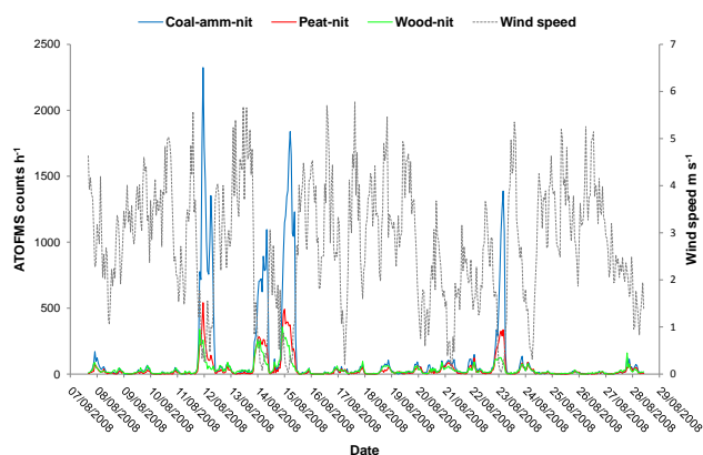
Fig. 7. Hourly integrated ATOFMS particle counts for the Coal-amm-nit, Peat-nit and Wood-nit subclasses and hourly averaged wind speed values for 7–28 August 2008.
