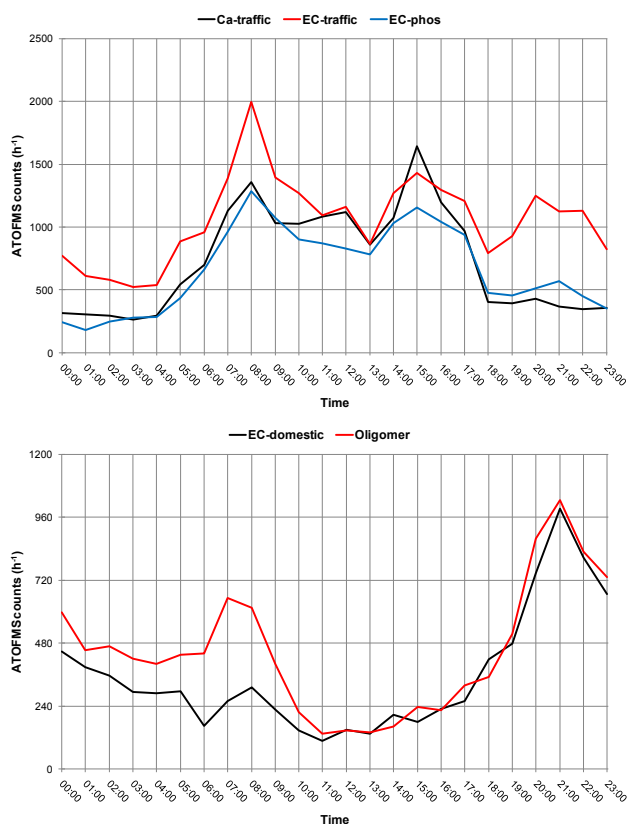
Fig. 11. Average diurnal trend for (top) Ca-traffic, EC-traffic and EC-phos and (bottom) EC-domestic and Oligomer particle counts for 7–28 August 2008. EC-phos and EC-domestic particle numbers have been multiplied by a factor of 3 and 1.5 respectively for comparative purposes.
