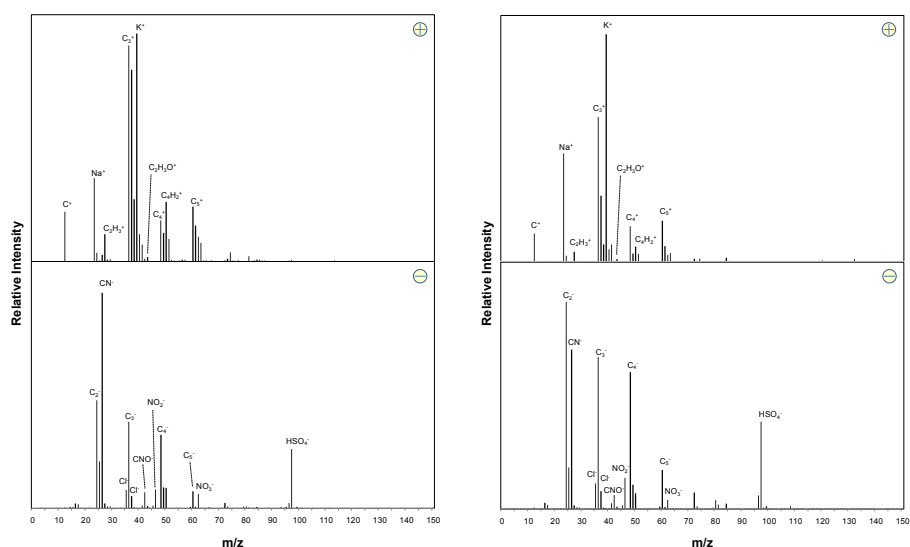
Fig. 3. Average dual ion mass spectra of ambient particles classified as “Peat” (left) and particles sampled during the peat combustion experiment (right).
