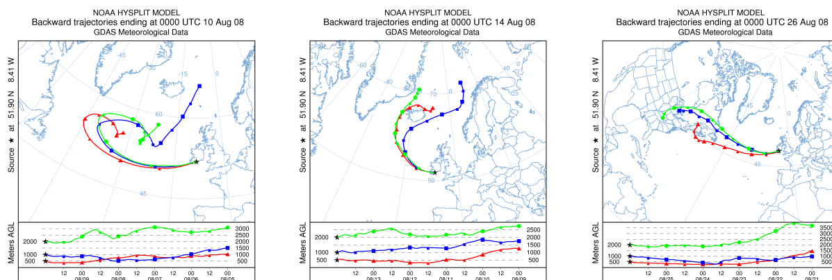
Fig. 15. 5 day back-trajectories for air masses arriving at Cork Harbour at 00:00 on 10 (left), 14 (middle) and 26 August 2008 (right).
