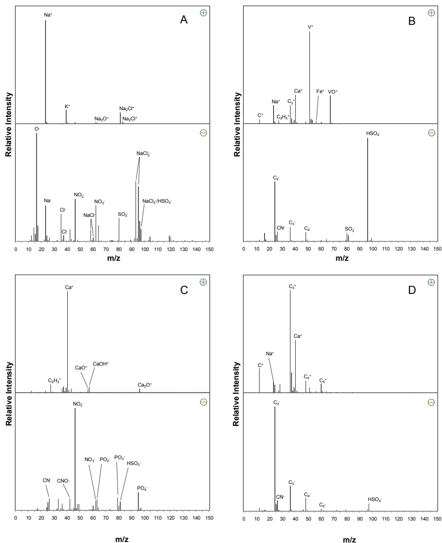
Fig. 10. Average dual ion mass spectra of ATOFMS particle classes; (A) Sea salt, (B) Shipping, (C) Ca-traffic, (D) EC-traffic.
