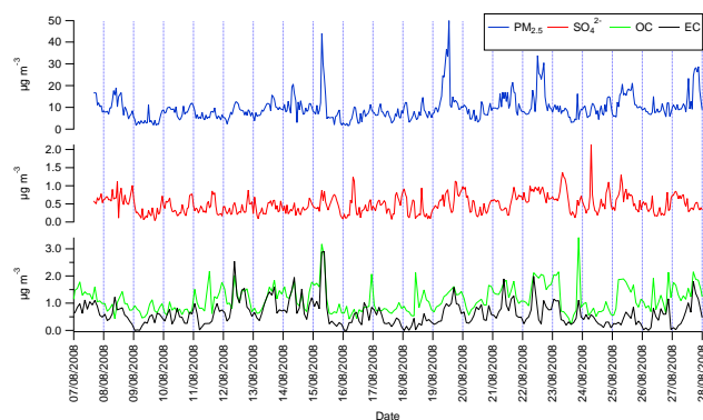
Fig. 2. Concentration-time profiles for PM 2.5 * , SO 4 2- * , organic carbon ** and elemental carbon ** for 7–28 August 2008. * Hourly averaged mass concentration. ** Bihourly averaged mass concentration.
