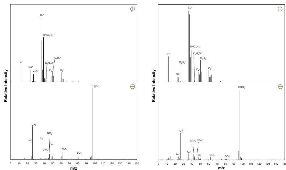
Fig. 4. Average dual ion mass spectra of ambient particles classified as “Coal” (left) and particles sampled during the coal combustion experiment (right).
