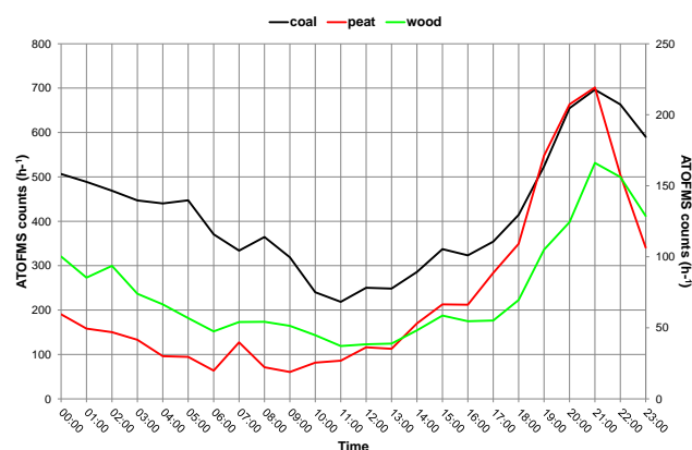
Fig. 6. Average diurnal trend for Coal, Peat and Wood ATOFMS particle counts for 7–28 August 2008.
