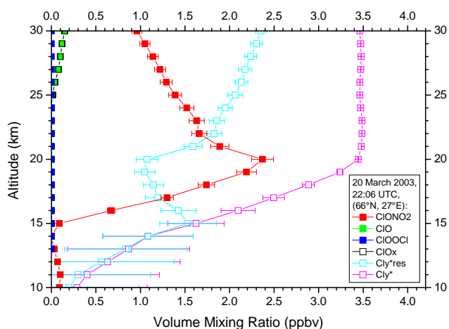
Fig. 12. Chlorine species as measured by MIPAS-B on 20 March 2003 inside the Arctic vortex. Notation as per Fig. 11. Deactivation of active chlorine is expressed by high \text{ClONO}_2 values around 20 km. \text{ClOOCl} values were set to zero for the calculation of \text{Cl}_y^* since \text{ClOOCl} was well below the detection limit.
