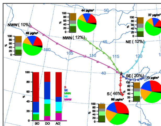
Fig. 5. The back trajectory clusters associated the corresponding average PM 1 compositions during the campaign. The inserted bar graph shows the directional variation of BTs before the Olympics (BO, 23 July–7 August), during the Olympics (DO, 8–24 August) and after the Olympics (AO, 25 August–20 September).
