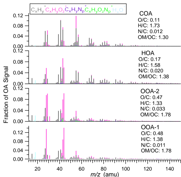
Fig. 3. The MS profiles of the four OA components of this study identified by PMF.
