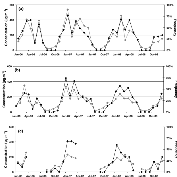
Fig. 8. Monthly mean concentrations (black) and monthly frequencies of daily concentrations higher than 150 \mu\text{g m}^{-3} (grey) in Banizoumbou (a), Cinzana (b) and M'Bour (c) from January 2006 to December 2008 (For M'Bour, values are given only if the number of daily data per month is higher than 15).
