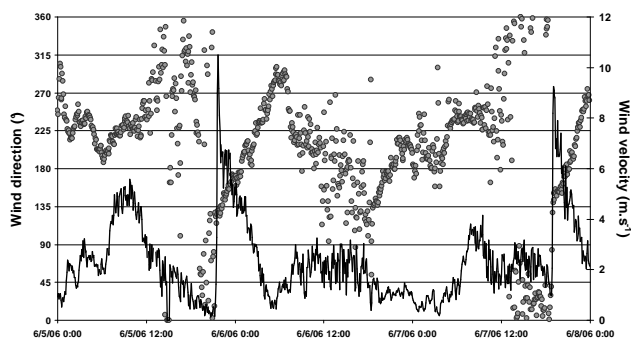
Fig. 13. 5-min surface wind directions (grey dots) and velocities (black line) measured in Cinzana from 5 to 8 June 2006.
