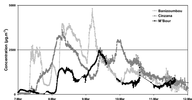
Fig. 10. 5-min mean \text{PM}_{10} concentrations measured in Banizoumbou (Niger), Cinzana (Mali) and M’Bour (Senegal) from 7 to 12 March 2006.
