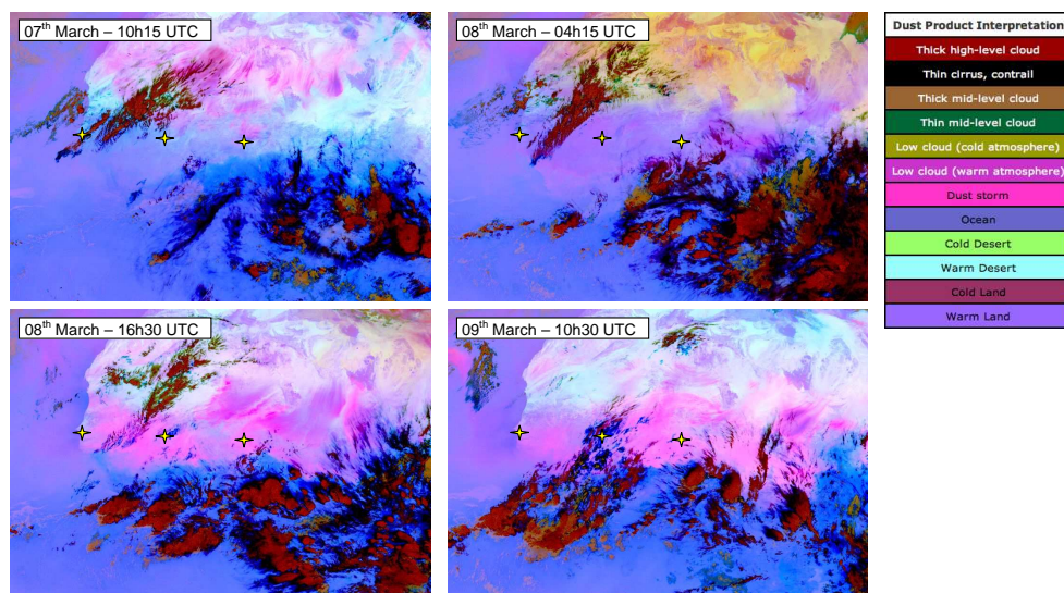
Fig. 11. SEVIRI special dust and pseudo visible products generated using Eumetsat algorithm and data from Eumetsat (infrared channels 12.0, 10.8 and 8.7 mm) of the SEVIRI by the RADAGAST Team (Radiative Atmospheric Divergence using Arm mobile Facility, GERB and AMMA stations): on 7 March 2006 at 10:15, on 8 March 2006 at 04:15 and 16:30 and on 9 March 2006 at 10:30. Dust appears pink or magenta and thick high-level clouds appear in red-brown, showing the presence of convective systems. The yellow stars represent the stations of M'Bour (left), Cizana (center) and Banizoumbou (right).
