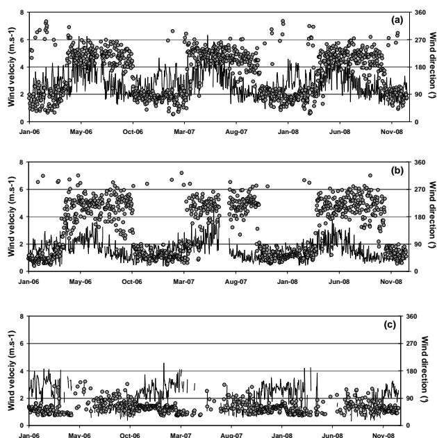
Fig. 6. Daily mean surface wind velocity (line) and daily wind direction (dots) in Banizoumbou (a), Cinzana (b) and M'Bour (c) from January 2006 to December 2008 (note that the wind velocities are lower in Cinzana due to a lower position of the wind sensor).
