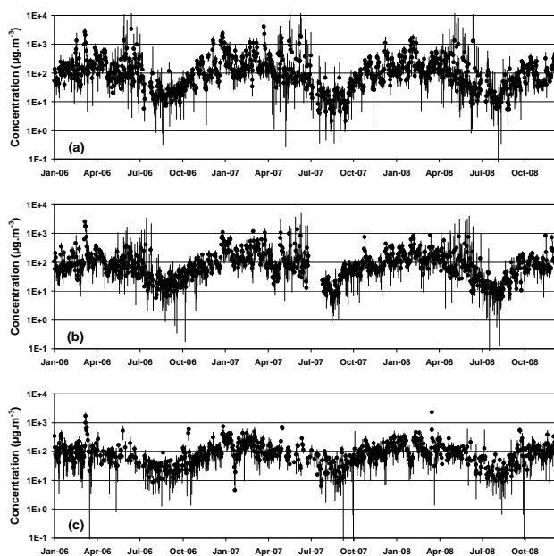
Fig. 3. Daily mean \text{PM}_{10} concentration and standard deviation in Banizoumbou (a), Cinzana (b) and M'Bour (c) for the selected "dust" wind sectors.
