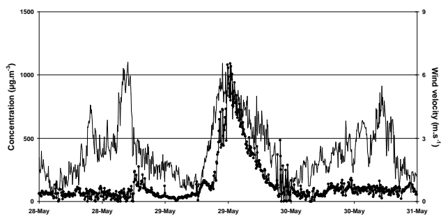
Fig. 12. 5-min PM_{10} concentrations (black dots) and surface wind velocities (black line) measured in M'Bour from 28 to 31 May 2006.
