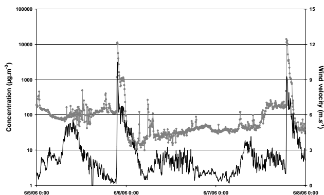
Fig. 15. 5-min surface wind velocities (black line) and \text{PM}_{10} concentrations measured in Cinzana from 5 to 8 June 2006.
