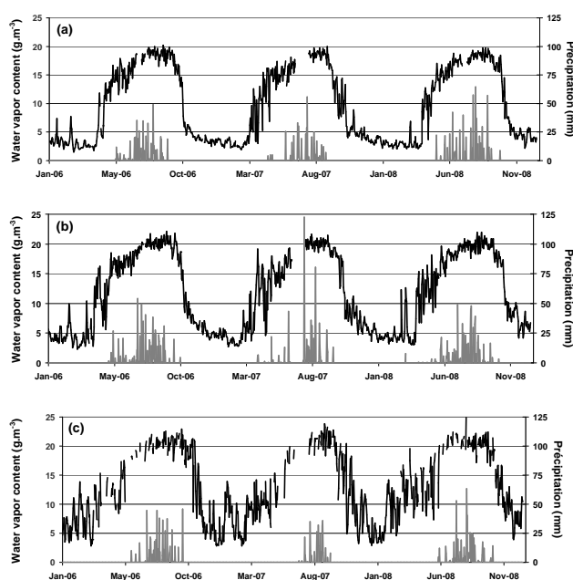
Fig. 5. Daily mean air humidity (black) and daily precipitation (dark grey) measured in Banizoumbou (a), Cinzana (b) and M'Bour (c) from January 2006 to December 2008.
