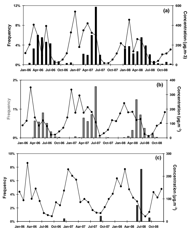
Fig. 7. Monthly frequency of high wind speeds (black bars : > 7 \text{ m s}^{-1} ; grey bars : > 6 \text{ m s}^{-1} ) and monthly mean concentration of dust (black line with black circles) in Banizoumbou (a), Cinzana (b) and M'Bour (c) from January 2006 to December 2008.
