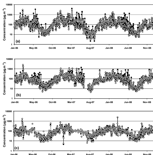
Fig. 4. Daily mean (black circle) and median (open circle) concentrations and 30-days sliding average on the daily mean (grey line) in Banizoumbou (a), Cinzana (b) and M'Bour (c) from January 2006 to December 2008.
