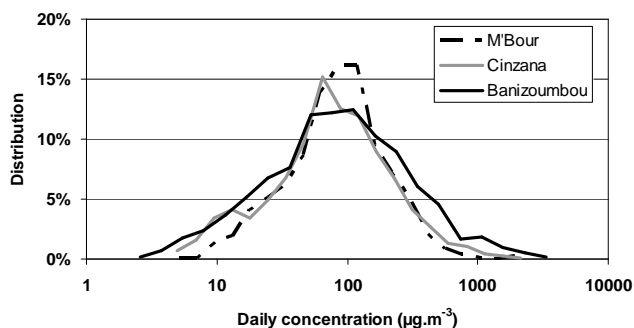
Fig. 2. Relative distribution of the daily mean \text{PM}_{10} concentrations from the three stations of the SDT between January 2006 and December 2008.
