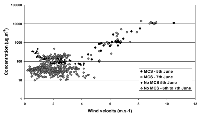
Fig. 16. 5-min \text{PM}_{10} concentrations as a function of the 5-min surface wind velocities measured in MCS and no MCS conditions in Cinzana from 5 to 8 June 2006.
