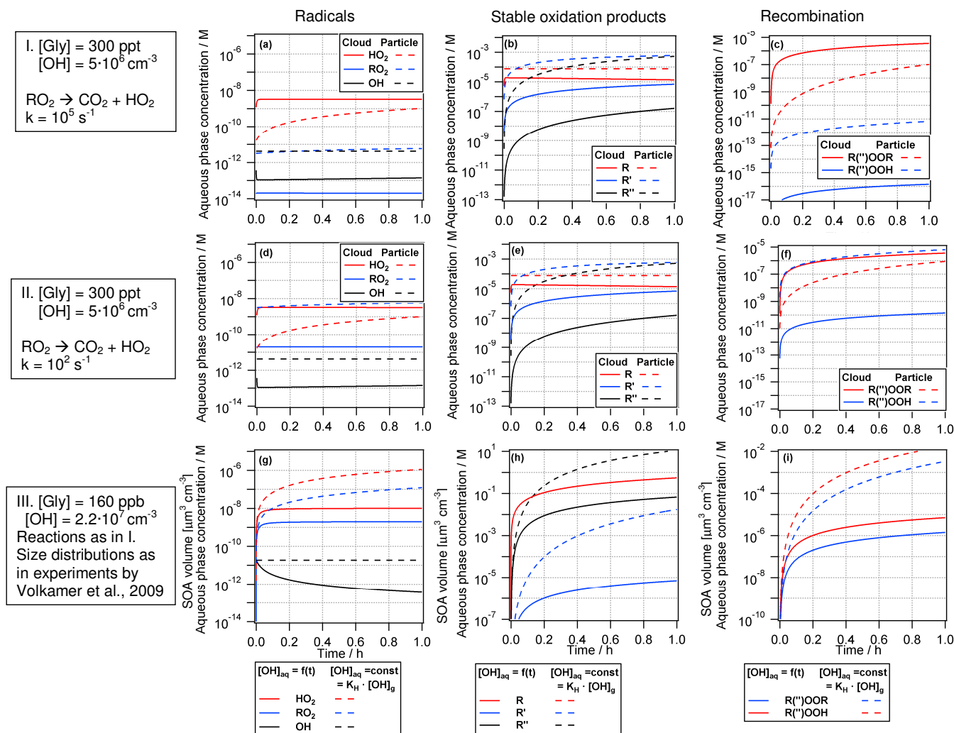
Fig. 3. Predicted concentration profiles of aqueous phase concentrations reactive intermediates (radicals) ( a, d, g ), stable oxidation products ( b, e, h ) and recombination products ( c, f, i ) simulated with the reaction scheme in Table 4. “Cloud” refers to dilute aqueous phase conditions with drop diameters D = 20 \mu\text{m} , \text{LWC} = 0.4 \text{ g m}^{-3} , N_{\text{droplets}} = 100 \text{ cm}^{-3} ; “particle” to a more concentrated aqueous phase with aqueous particles with diameters D = 100 \text{ nm} , \text{LWC} = 20 \mu\text{g m}^{-3} , N_{\text{particles}} = 5000 \text{ cm}^{-3} . Top panel (a–c): the decay rate of peroxy radicals has been assumed as 10^5 \text{ s}^{-1} (Table 4) (Neta et al., 1990). Middle panel (d–f): the decay rate of peroxy radicals has been assumed as 10^2 \text{ s}^{-1} (Table 4) (Neta et al., 1990). Bottom panel (g–i): same mechanism and rate constants as for top panel but initial gas phase concentrations as used in experiments by Volkamer et al. (2009) ( [\text{Glyoxal}]_{\text{gas}} = 160 \text{ ppb} ; [\text{OH}]_{\text{gas}} = 2.2 \times 10^7 \text{ cm}^{-3} ). [\text{OH}]_{\text{aq}} = f(t) includes the kinetic description of OH transfer into the aqueous phase (as used for all other simulations); [\text{OH}]_{\text{aq}} = \text{const.} assumes a constant OH concentration that implies thermodynamic equilibrium with the gas phase at all times [\text{OH}]_{\text{aq}} = K_{\text{H}}(\text{OH}) \cdot [\text{OH}]_{\text{gas}} (Sect. 3.3.1).
