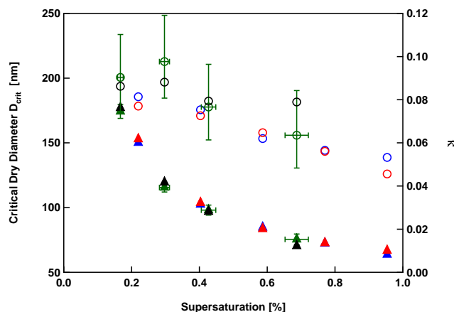
Fig. 8. Critical dry diameter for activation ( D_{\text{crit}} ) as a function of the supersaturation (solid triangles, left axis). Calculated \kappa from one parameters Köhler equation (open circles, right axis). The blue (080912) and black (080917) data was measured in the Ox.-induced experiments, red (080913) and green (080916) data stem from VOC-induced experiments. (Numbers in parenthesis refer to the experiment date). Typical errors are indicated for some cases. All data 6 to 7 h after the first nucleation started and the second nucleation mode is present. The \kappa are larger at small supersaturations where particles with larger diameter (and more aged) are probed.
