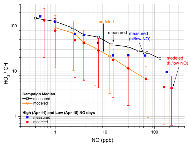
Fig. 4. The HO 2 /OH ratio as a function of NO. For graphical purposes, all of the HO x ratios are binned based on ranges of NO concentrations. We used the following bins: 0–1 ppb, 1–2 ppb, 2–3 ppb, 3–5 ppb, 5–10 ppb, 10–20 ppb, 20–40 ppb, 40–100 ppb, and 100–200 ppb. Each circle or square represents the median of each NO concentration bin. The predicted values from the model on a campaign median basis are shown as the orange line with open circles, whereas the median measured values from the entire campaign are shown as a black line with open squares. The closed red circles and closed blue squares are the modeled and measured HO x ratios, respectively, for the high and low NO days, 11 and 18 April. Note that the lines are not a fit through the symbols, but rather connect the symbols to help guide the eye.
