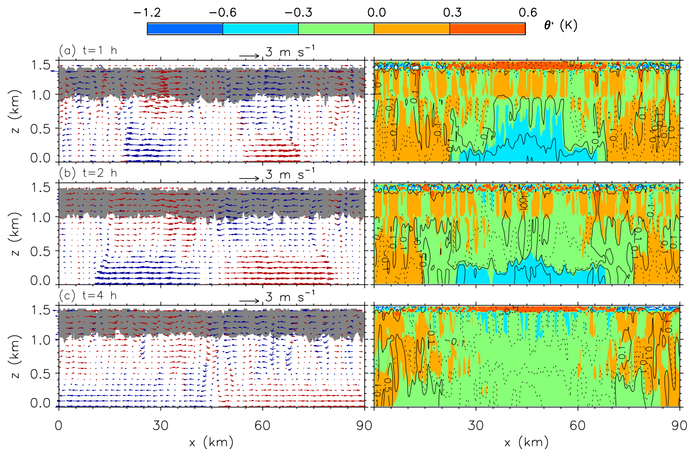
Fig. 7. The x - z cross-sections (at y=45 km) from experiment PQVT at (a)–(c) t=1, 2 and 4 h. Left: Gray shaded areas denote clouds (cloud water mixing ratio > 0.01 \text{g kg}^{-1} ); arrows represent wind perturbations ( u-w ) with red for westerly ( u>0 ) and blue for easterly ( u<0 ) to demonstrate the outflow at the lower-level and return flow at the upper-level associated with the negative temperature perturbation in the middle of the domain (originally between x=30 and 60 km). Right: Shaded colors indicate temperature perturbations, and contours, water vapor mixing ratio perturbations (positive by solid lines and negative by dotted lines); perturbations are relative to the horizontal slab average at each level.
