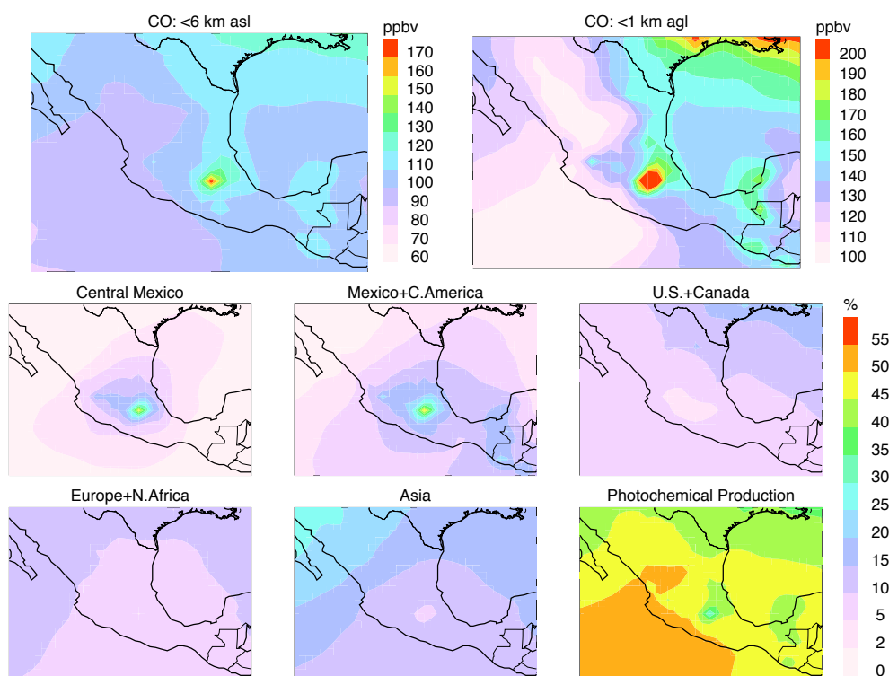
Fig. 7. Top, left: CO averaged for 1–31 March 2006 over the tropospheric column (surface to 6 km, or 400 hPa, a.s.l.); top right: same, averaged over the lowest km above the surface. Middle and bottom rows: fraction of tagged CO to total CO averaged over the tropospheric column.
