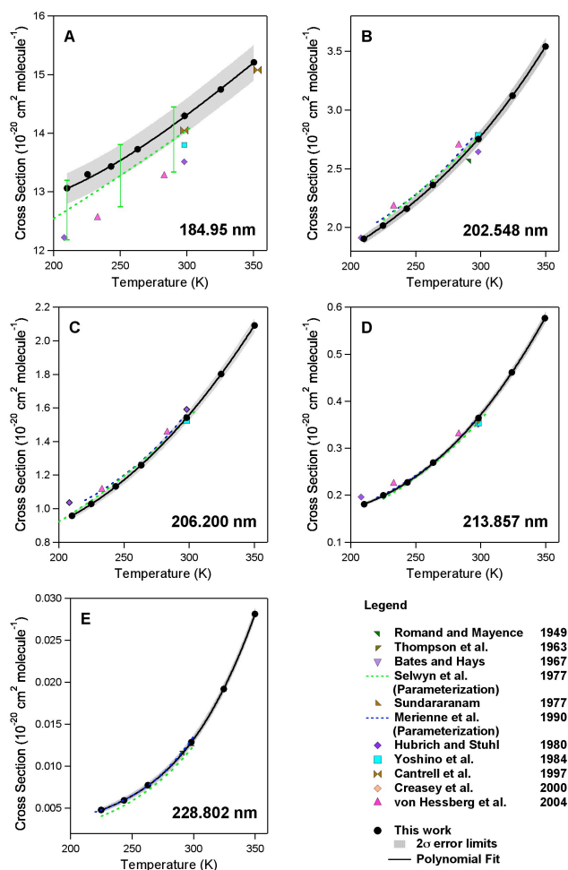
Fig. 2. Temperature dependent N 2 O absorption cross sections obtained in this work (●). The shaded region represents the estimated absolute 2 \sigma (95% confidence level) uncertainty from our work including estimated systematic errors. Included for comparison are results from previous studies as indicated in the legend. The data from Mérienne et al. (1990) and Selwyn et al. (1977) are plotted using the cross section and temperature dependence parameterizations reported in their work. Data from Zelikoff et al. (1953) are not included due to their large deviation from the other studies. The results from Selwyn et al. (1977) supersedes the results from Johnston and Selwyn (1975), which are not shown.
