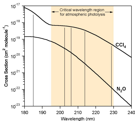
Fig. 1. The JPL06-2 (Sander et al., 2006) recommended UV absorption cross section spectra of N 2 O and CCl 4 at 298 K. The shaded area highlights the wavelength region most important for atmospheric photolysis. The vertical lines correspond to the wavelengths of the atomic lines used in this work.
