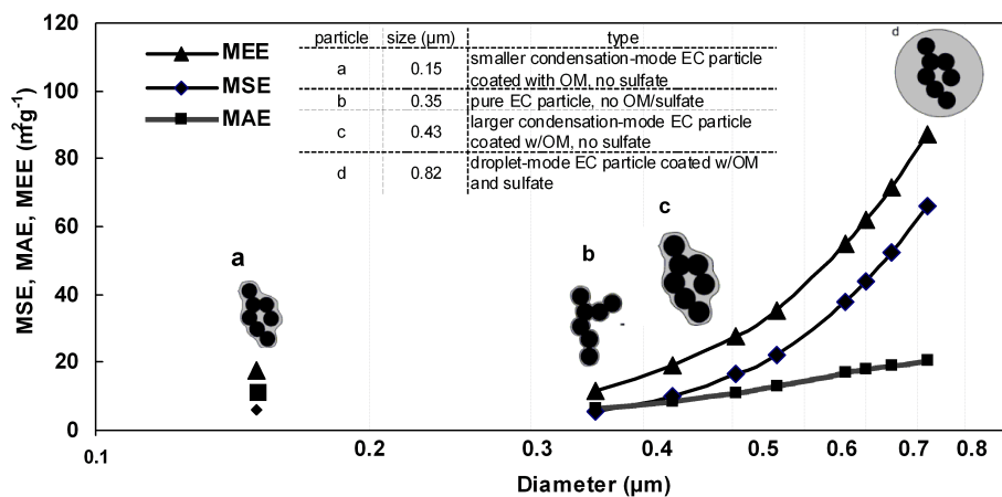
Fig. 3. EC-normalized mass scattering efficiency (MSE), mass absorption efficiency (MAE) and mass extinction efficiency (MEE) of four types of EC-containing particles, taking chemical composition of the HKUST sample collected on 5–6 February 2008 as example.
