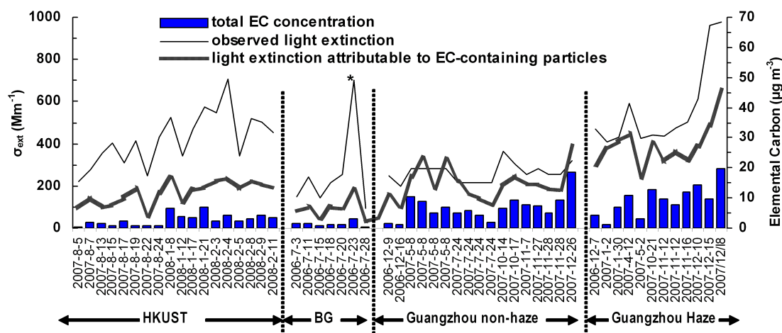
Fig. 4. Calculated and observed light extinction coefficients at the selected urban, suburban and rural locations in the Pearl River Delta region. An episodic biomass burning event occurred nearby the rural sampling site on the sampling day marked with *.
