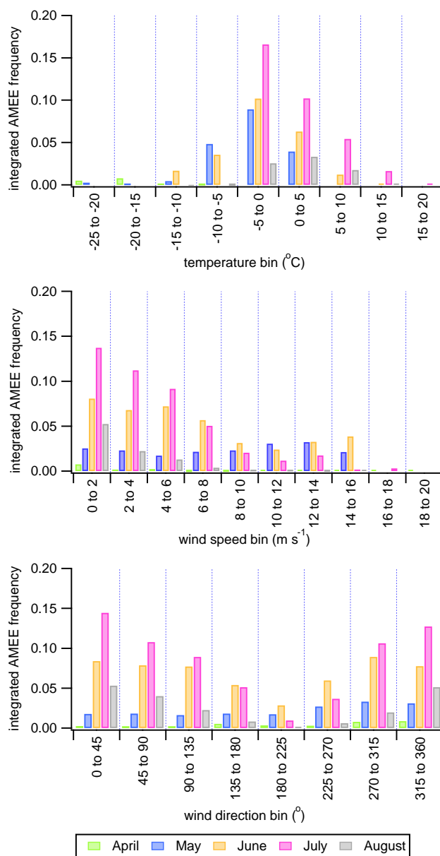
Fig. 4. Integrated atmospheric mercury emission event frequency ( F_{AMEE} ) as a function of temperature, wind speed, wind direction and month for Alert data 1995–2007. Note the change in scale from Figs. 2 and 3.
