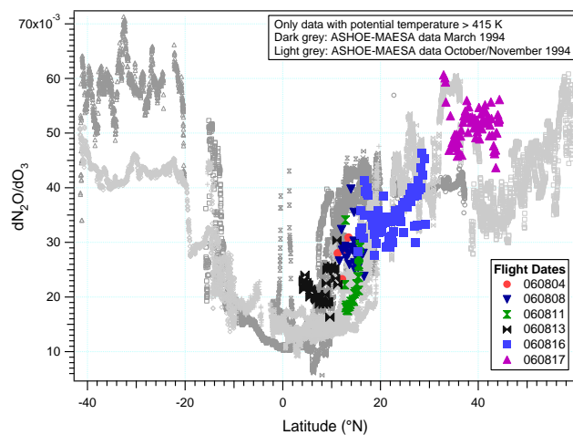
Fig. 12. Slope dN_2O/dO_3 against latitude for the AMMA/SCOUT-O3 (coloured) and ASHOE/MAESA (grey) flights.
