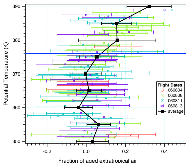
Fig. 8. Fraction of aged extratropical air. The blue line represents the average height of the tropopause.
