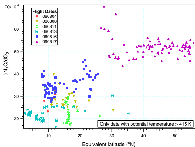
Fig. 11. Slope dN_2O/dO_3 against equivalent latitude for the AMMA/SCOUT-O3 flights.
