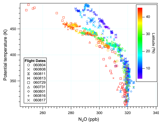
Fig. 7. Vertical profile of N 2 O coloured to latitude.
