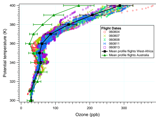
Fig. 3. Ozone profiles for the five local flights. The average profile is indicated with the black line. The green line represents the average ozone profile for the SCOUT-O3 campaign over Australia in November/December 2005.
