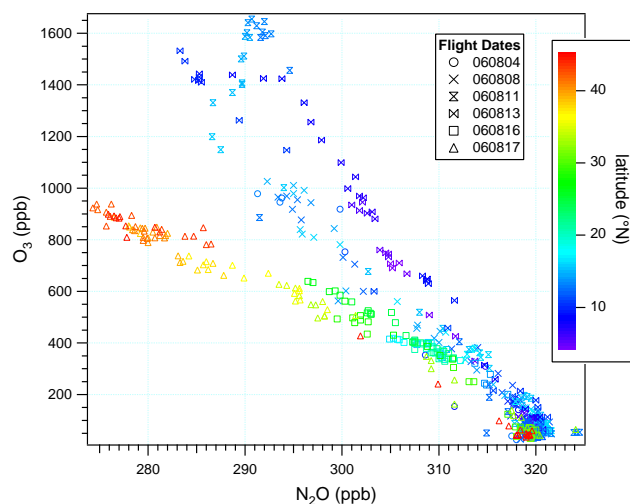
Fig. 9. Correlation between N_2O and O_3 coloured to latitude.
