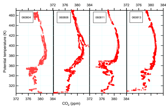
Fig. 2. Potential temperature profiles of CO 2 for the flights on 4, 8, 11 and 13 August, respectively.
