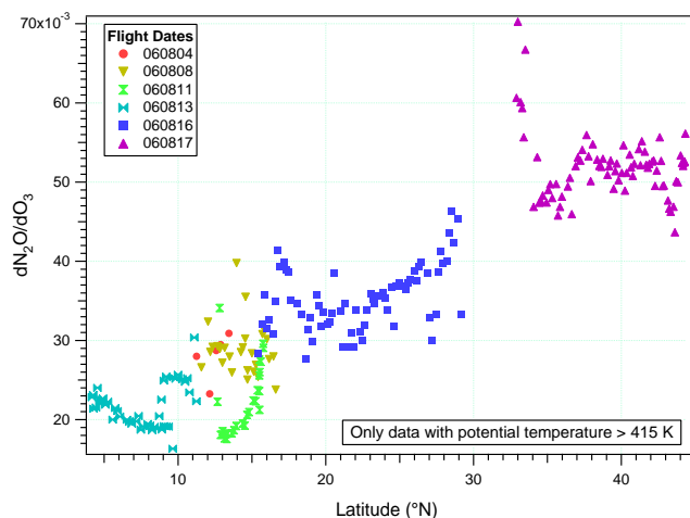
Fig. 10. Slope dN_2O/dO_3 against latitude for the AMMA/SCOUT-O3 flights.
