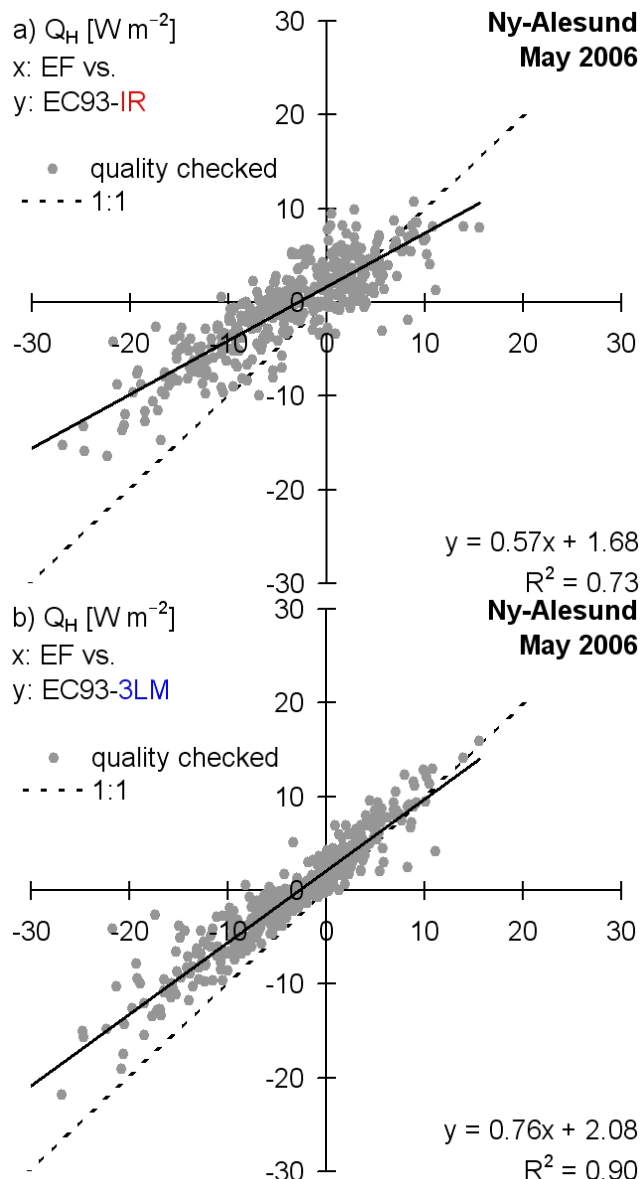
Fig. 4. Linear correlation of the sensible heat flux Q_H [ \text{W m}^{-2} ] measured with a sonic-anemometer applying the eddy-covariance method (EF), and calculated with the EC93-parameterization (Ebert and Curry, 1993) over a snow surface using (a) the IR-derived (IR) and (b) the 3-layer-model-extrapolated (3LM) surface temperature T_{(0)} as input. Quality checked values, elimination of the periods with non-stationary conditions (steady state test) and snowdrift or precipitation effects on the sonic-anemometer, 7 May to 19 May 2006. Ny-Ålesund (Svalbard), ARCTEX-2006.
