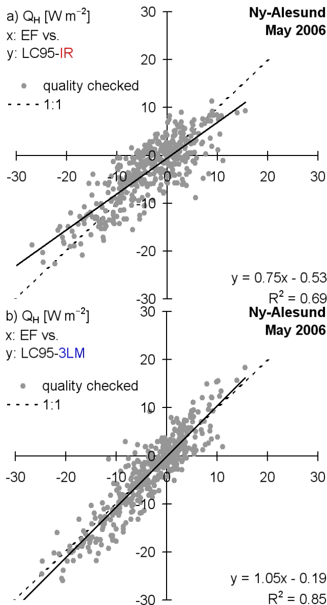
Fig. 3. Linear correlation of the sensible heat flux Q_H [ \text{W m}^{-2} ] measured with a sonic-anemometer applying the eddy-covariance method (EF), and calculated with the LC95-parameterization (Lau and Cheng, 1995) over a snow surface using (a) the IR-derived (IR) and (b) the 3-layer-model-extrapolated (3LM) surface temperature T_{(0)} as input. Quality checked values, elimination of the periods with non-stationary conditions (steady state test) and snowdrift or precipitation effects on the sonic-anemometer, 7 May to 19 May 2006. Ny-Ålesund (Svalbard), ARCTEX-2006.
