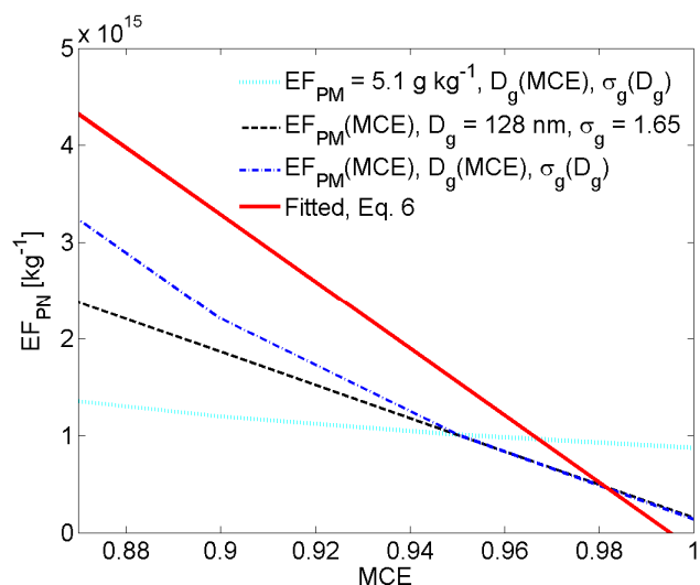
Fig. 5. Particle number emission factors ( EF_{PN} ) related to dry mass burned versus modified combustion efficiency ( MCE ), calculated from the particle mass emission factor for the overall data set ( EF_{PM,overall} ). EF_{PM,overall} is either constant at MCE=0.95 ; EF_{PM,overall}=5.1 \text{ g kg}^{-1} d.m., or varied with MCE , Eq. (10). The particle sizes are either constant at MCE=0.95 ; D_g=128 \text{ nm} and \sigma_g=1.65 , or varied with MCE , Eqs. (2–3).
