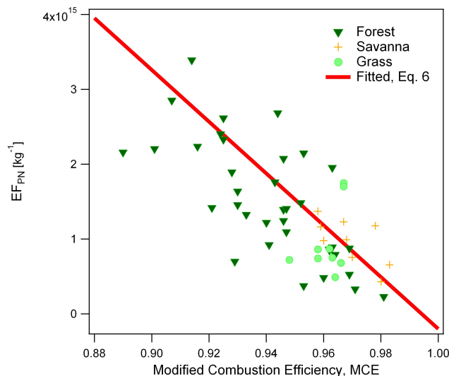
Fig. 2. Particle number emission factors ( EF_{PN} ) related to dry mass burned versus modified combustion efficiency (MCE) for three fuel types; forest (Guyon et al., 2005; Kuhn et al., 2010), and savanna and grass (Le Canut et al., 1996). A standard fitting method is used on the overall data set to find EF_{PN}/[\text{kg}^{-1}] = (34.4 \times 10^{15} - 34.6 \times 10^{15} \times \text{MCE}) \pm 0.8 \times 10^{15} , Eq. (6), shown as a line. Measurements for savanna and grass data used a \sim 100 nm particle diameter detection limit and have been corrected as described in Sect. 4.1.
