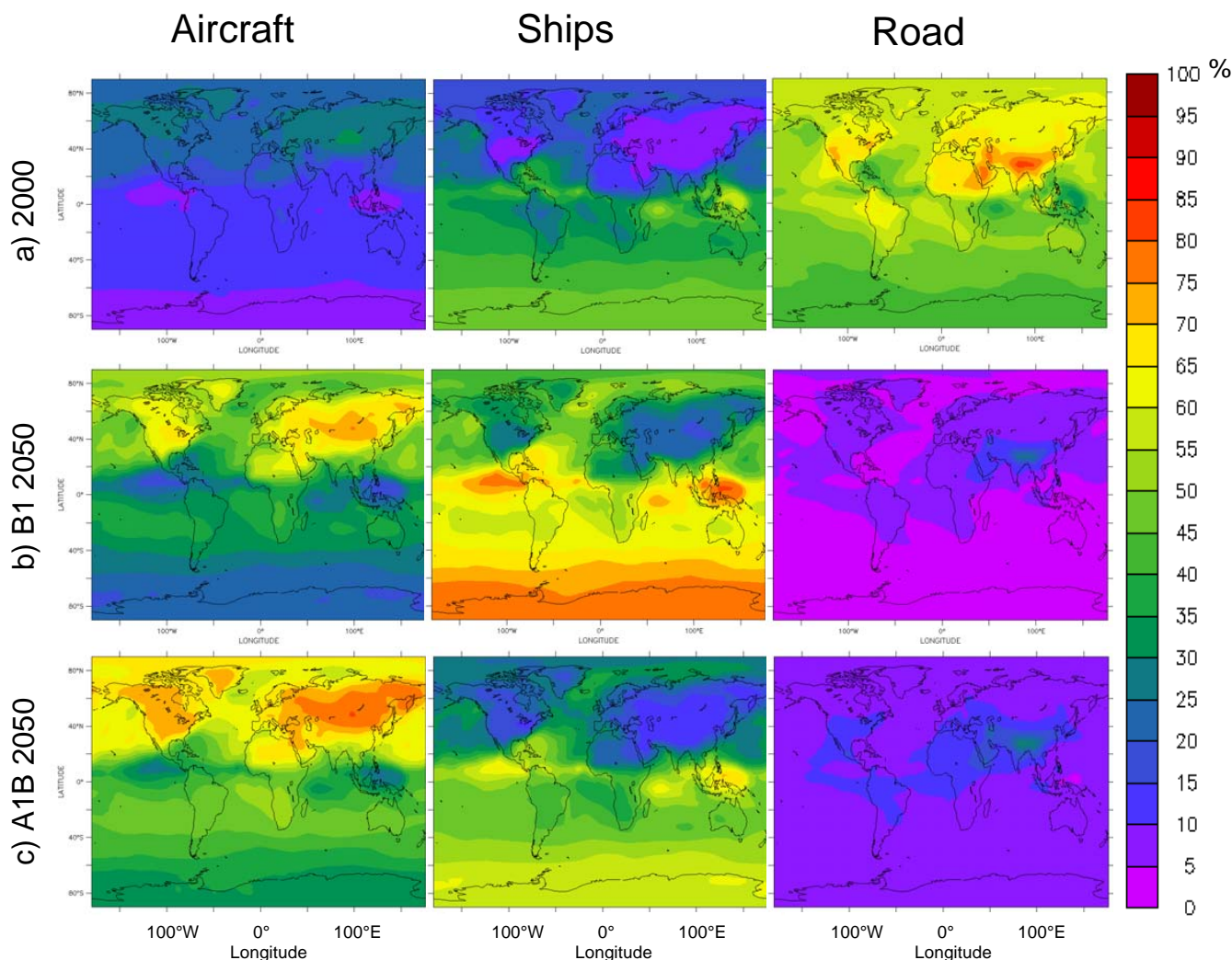
Fig. 2. Respective contribution (%) of each transport mode to the tropospheric ozone column change due to transport in July, for 2000 (A experiment) and 2050 (B1 and A1B scenarios; B and C experiments, respectively) emissions.
