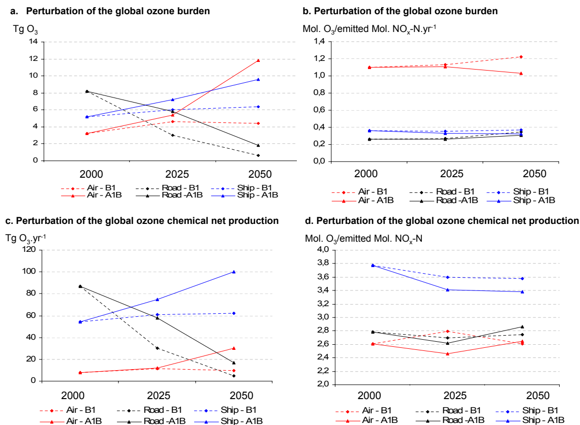
Fig. 7. Perturbation of the global ozone burden ( a, b ) and the global ozone chemical net production ( c, d ) due to 2000, 2025 and 2050 emissions from aircraft, road traffic and shipping. Both the absolute (left) and the relative (mol. O 3 per mol. of emitted NO x ; right) perturbations are presented.
