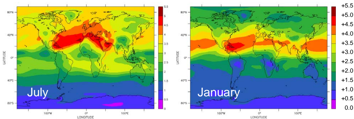
Fig. 10. Up-scaled tropospheric ozone column perturbation ( \Delta DU) due to (a) 2000 transport emissions in a present climate and (b) 2050 transport emissions in a present climate, (c) 2050 transport emissions in a future climate, as simulated for July (left) and January (right) conditions (A1B emission scenario).
