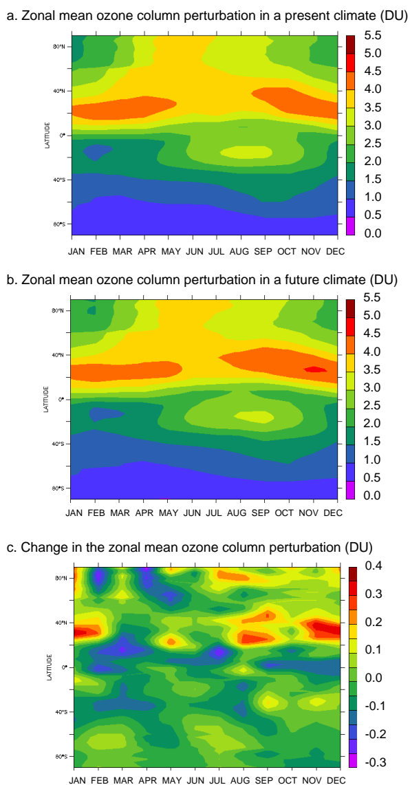
Fig. 12. Impact of transport emissions on the zonal mean tropospheric ozone column (a) in a present and (b) in a future (A1B scenario, 2050) climate, and (c) corresponding change ( \Delta DU).
