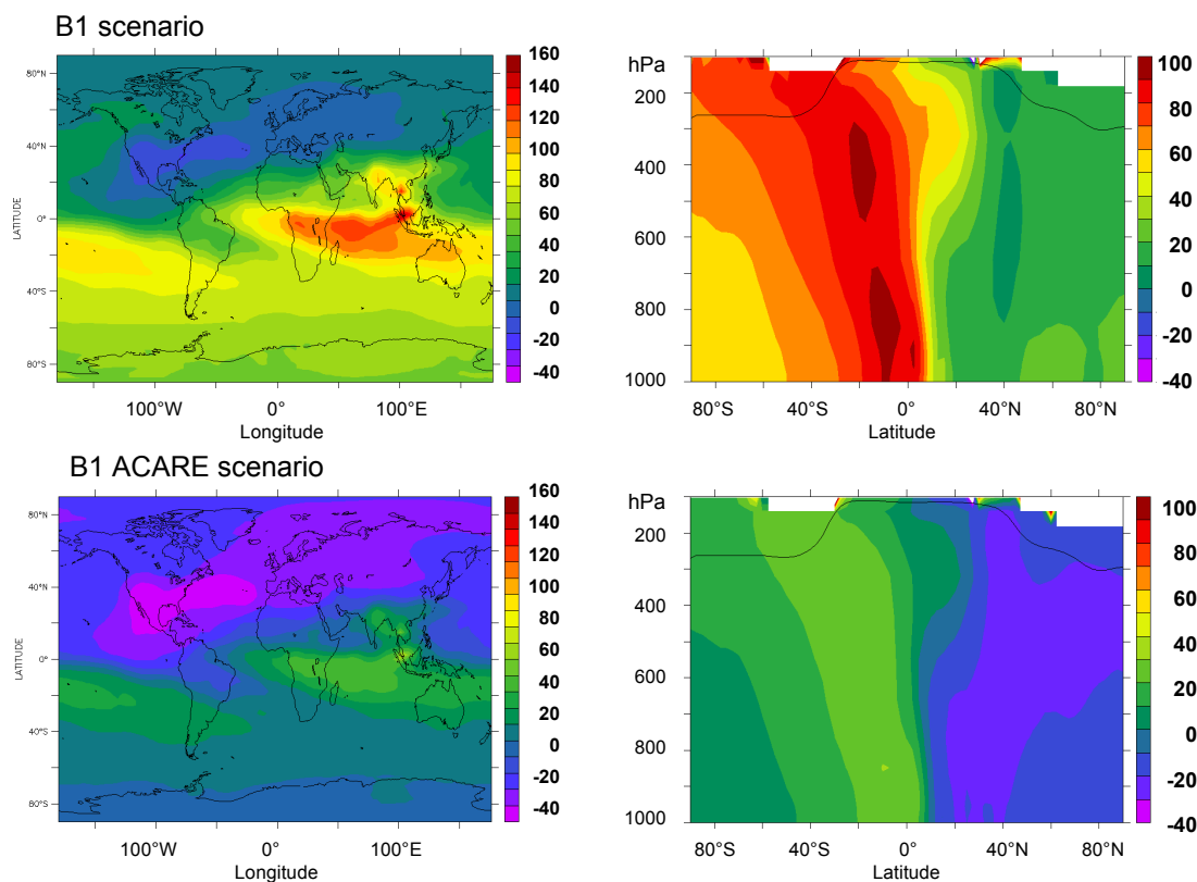
Fig. 6. (a) Perturbations in zonal mean ozone mixing ratio (in %) due to aircraft emissions, for July from 2000 (left), 2050 B1 (middle) and 2050 B1 ACARE (right) emissions; (b) 2000–2050 changes (%) in the O_3 tropospheric column and zonal mean ozone perturbations by aircraft emissions for B1 scenario, and (c) B1 ACARE scenario.
