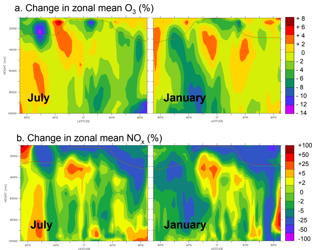
Fig. 9. Future change in O 3 (%) and NO x (%) zonal mean mixing ratio, for July (left) and January (right) conditions (A1B emission scenario).
