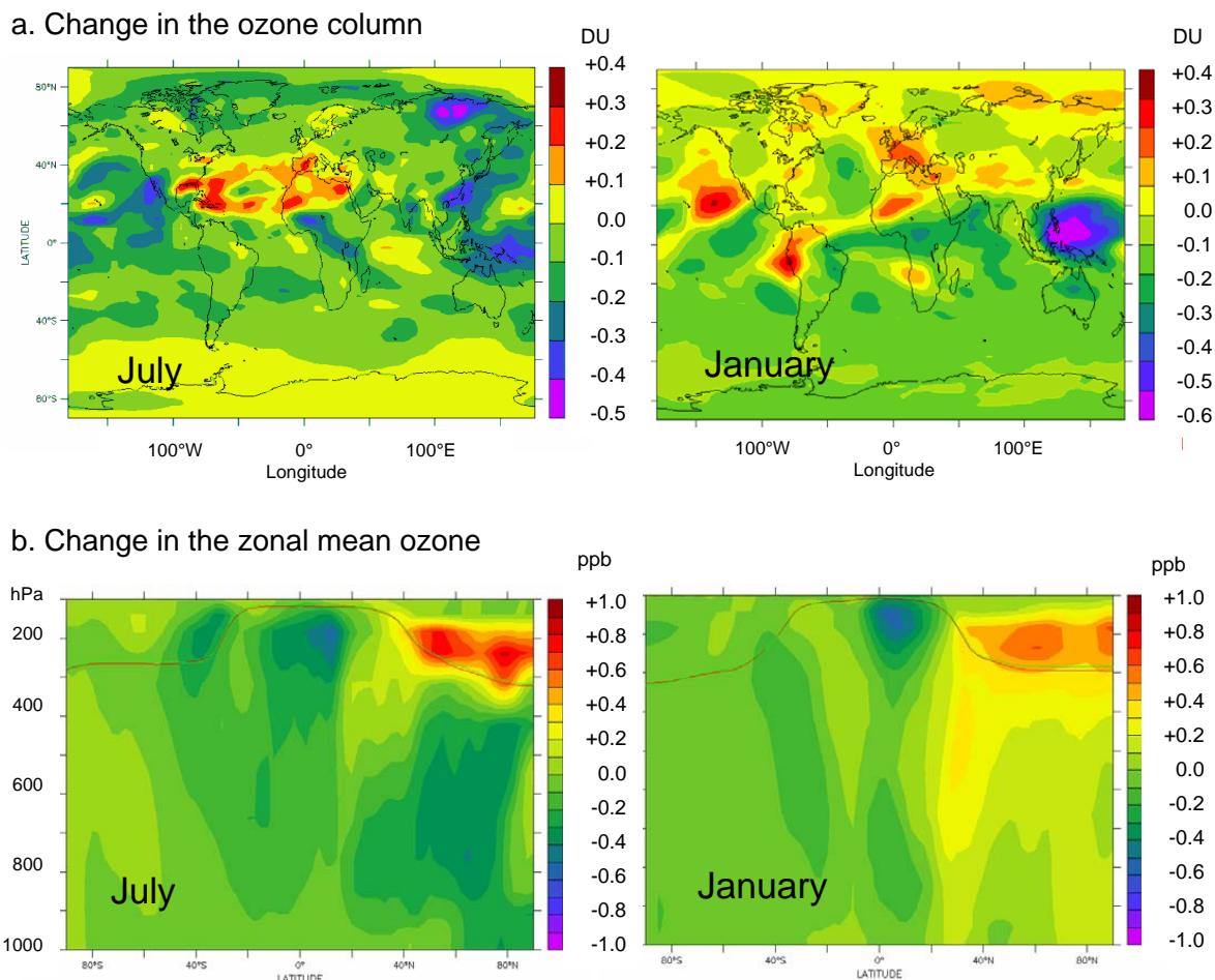
Fig. 11. Effect of future (2050) climate change on the impact of transport emissions on (a) the tropospheric ozone column ( \Delta DU) and (b) on zonal mean ozone mixing ratio ( \Delta ppb v ) for July (left) and January (right) conditions (A1B scenario).
