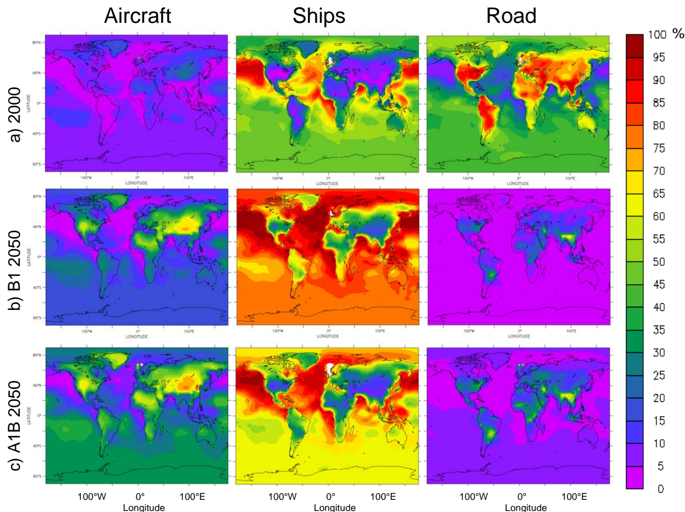
Fig. 3. Same as Fig. 2 for surface ozone mixing ratio.
