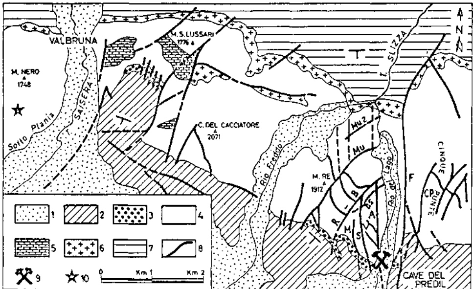
Fig. 1: Generalized geologic map of the Raibl (Cave del Predil) - Valbruna area (Assereto and Brigo, 1978). Explanation: 1. Quaternary; 2. Carnian: upper part of the Calcare del Predil Formation and Rio del Lago, Rio Conzen and Tor Formations; 3. Lower Carnian: lowermost part of the Clacare del Predil Formation; 4. Ladinian-Carnian: Dolomia Metallifera; 5. Ladinian-Carnian: "Buchenstein" intercalated within the Dolomia Metallifera; 6. Lower Ladinian: Rio Freddo Volcanites; 7. Comprehensive Lower Ladinian + Anisian + Scythian Formations; 8. Faults (in the Raibl mine: R-B: Rinnengraben-Bärenklamm; BS: Bärenklamm Sud; M: Abendblatt-Morgenblatt; S: Struggl; A: Aloisi; V: Vincenzo; F: Fallbach; CP: Cinque Punte; Mu: Muda; Mu2: Muda 2); 9. Raiblmine; 10. Galena outcrops in the Dolomia Metallifera of the M. Nero (Valbruna).
