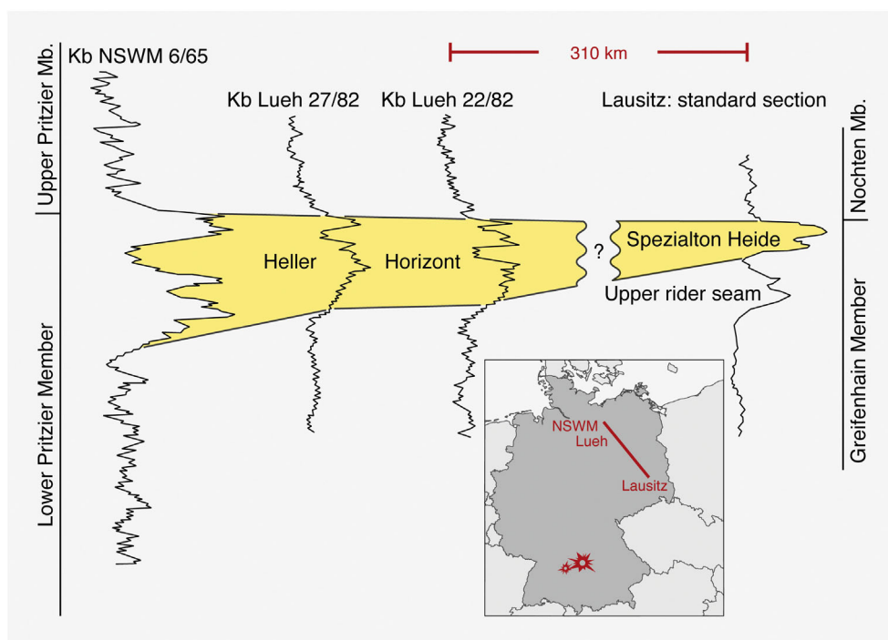
FIGURE 8. Correlation of gamma ray logging from boreholes in the Helle Horizon (bright horizon) and the Spezialton Heide (special clay of Heide).
