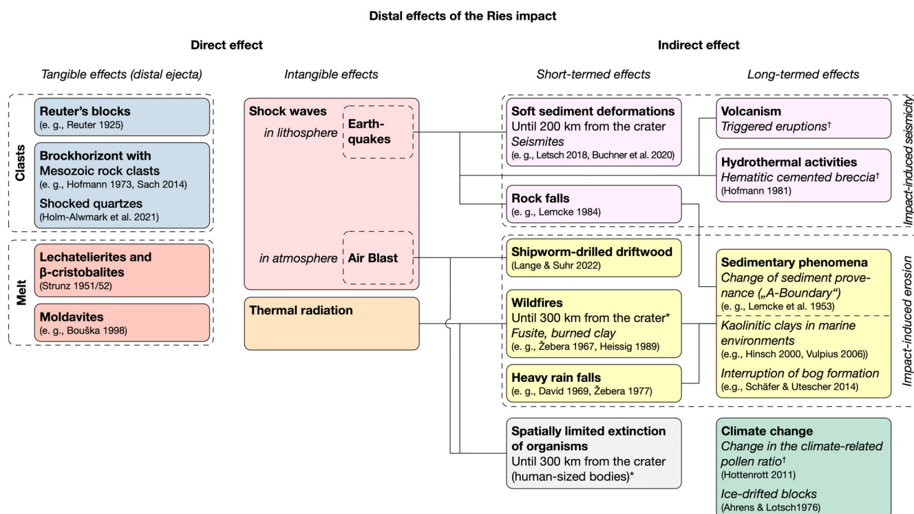
FIGURE 3. Summary of verified and presumed distal effects of the Ries impact. *Calculated by Collins et al. (2005), †not discussed in this work.
