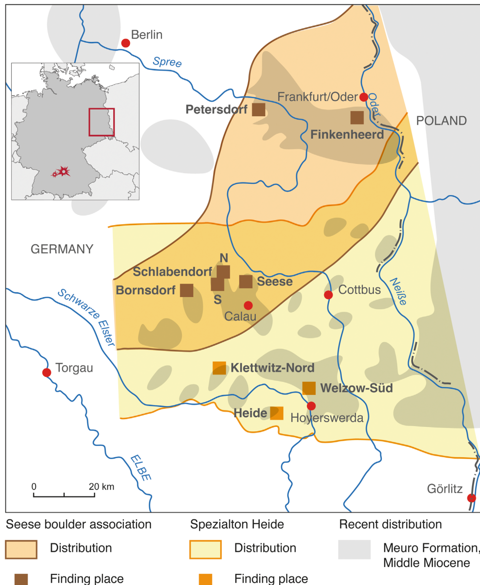
FIGURE 7. Distribution of the Seeser Gerölle (Seese boulders) and the Spezialton Heide (special clay of Heide) in the Lausitz area (modified after Ahrens & Lotsch, 1976).
