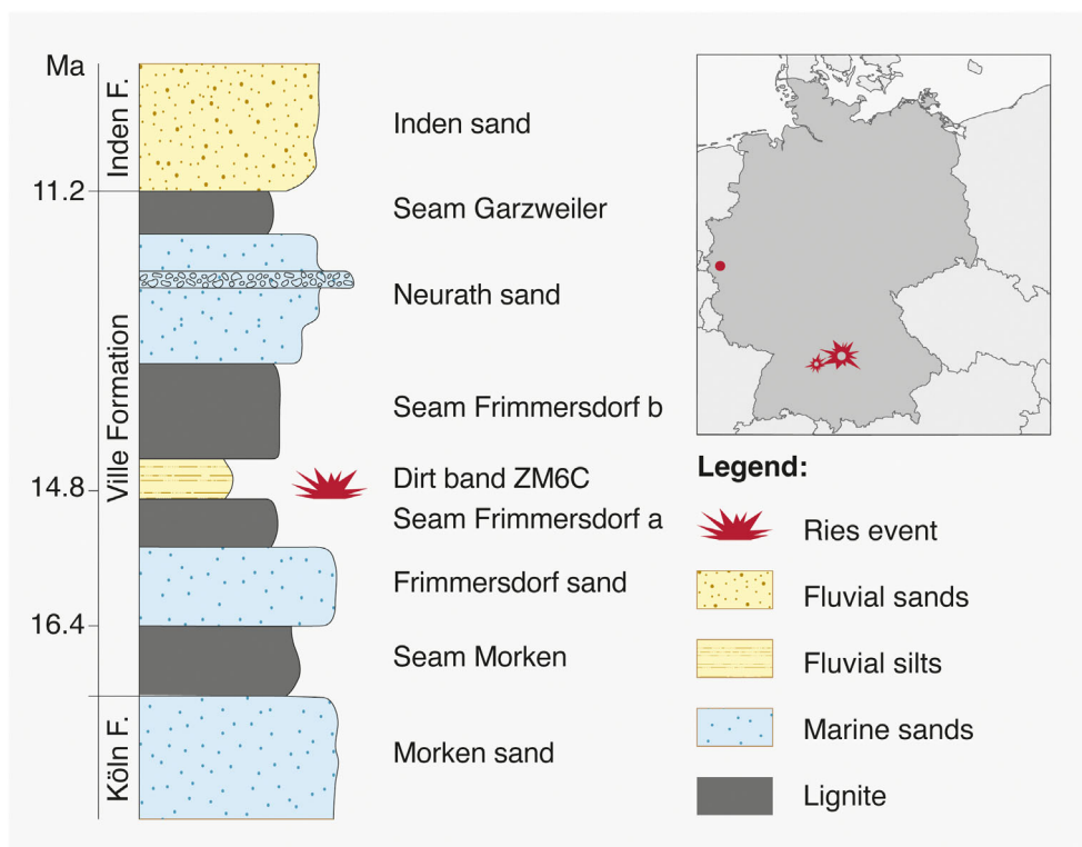
FIGURE 9. Profile of the Frimmersdorf seam from the Niederrhein lignite area (Ville Formation) with the fluvial dirt band ZM6C (following Schäfer & Utescher, 2014).
