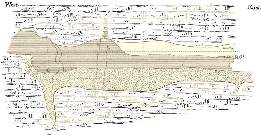
Fig. 2. Longitudinal Section of North side of Flint-Knife Gallery, into West Chamber L-L on Plan.
