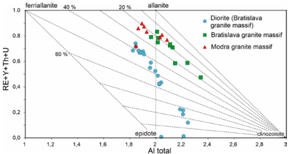
Fig. 6: Composition of allanite-(Ce) from diorites (BMD-1) and granodiorites (BMG-1) of the Bratislava granite massif and granodiorites of the Modra granite massif (MM-2).
