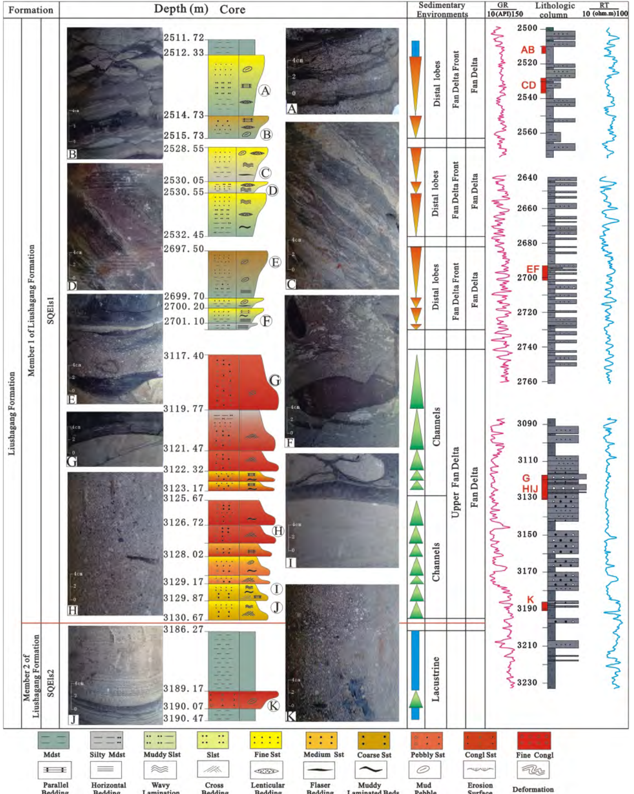
FIGURE 4: Macroscopic view of Well Fc1 cores. The 34.57 m cores in SQEs2 and SQEs1 occur from 3200 m to 2520 m.
