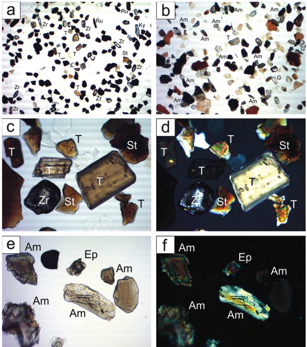
FIGURE 6: Photomicrographs of representative heavy mineral separates from different stratigraphic units found in the study area. a) HL 9/1, 2.5 times enlarged, b) HL 7/4.1, 2.5 times enlarged, c) OP 2/1, 10 times enlarged, d) OP 2/1, 10 times enlarged with crossed nicols, e) OP 2/5, 10 times enlarged, f) OP 2/5, 10 times enlarged with crossed nicols. Note the high relative amount of opaque grains and weathering-resistant minerals zircon (Zr), tourmaline (T) and rutile (Ru) in samples HL 9/1 and OP 2/1 assigned to the Cretaceous. Samples HL 7/4.1 and OP 2/5 from the Quaternary show lower amounts of opaque grains and higher amounts of less weathering-resistant minerals such as amphiboles (Am), garnets (G) and minerals of the epidote group (Ep). Cretaceous samples also show a better sorting compared to samples from the Quaternary. Ky - kyanite, St - staurolite, Sil - sillimanite.
