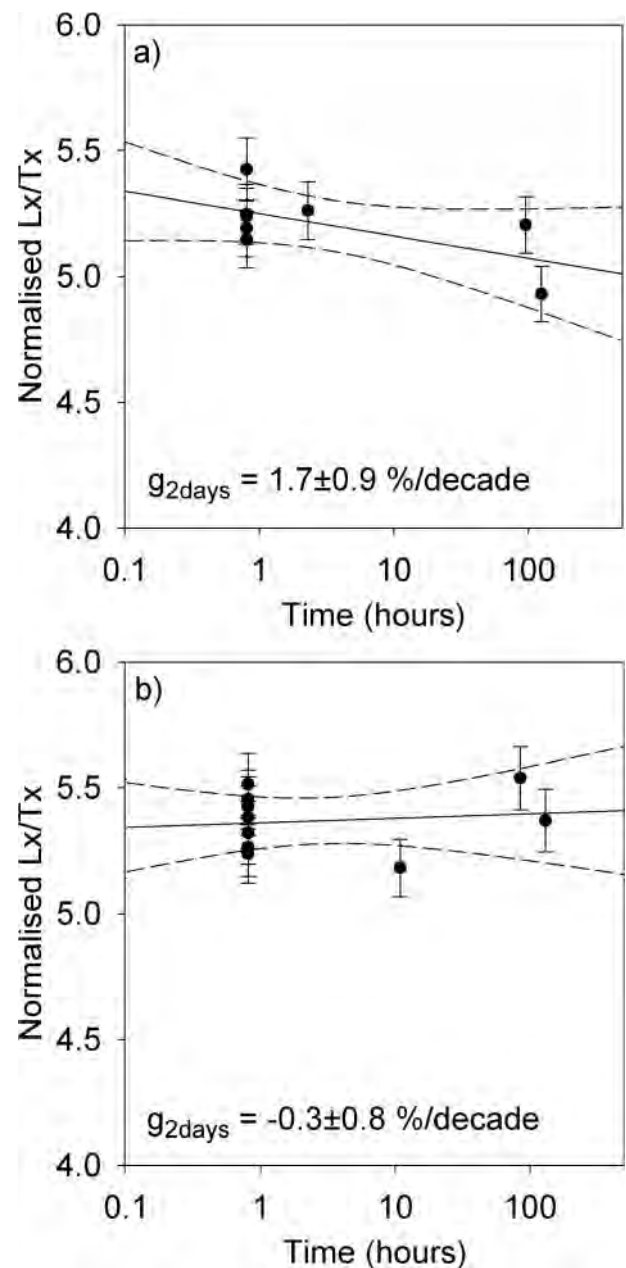
FIGURE 8: Fading test results for one fine-grained polymineral aliquot of sample A-KB 16/98 (32.2 m). Normalised (a) IRSL 50/225 and (b) pIRIR 225 Lx/Tx signal values are plotted against storage time. Dotted lines represent 2 sigma confidence intervals. Maximum storage times are (a) 125 h and (b) 130 h.
