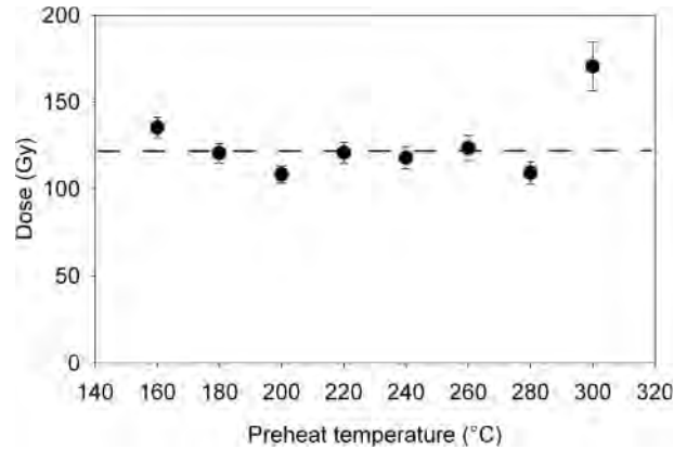
FIGURE 3: Representative results from a preheat plateau test performed on fine-grained quartz aliquots from sample A-KB 17/98 (31.6 m). Data points represent average values from three aliquots.
