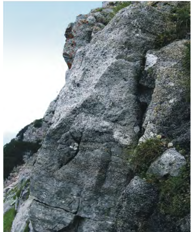
FIGURE 8: Fine-grained, calcite-cemented, well rounded and partly well sorted quartz conglomerate overlying fossiliferous limestone with erosive contact. Type section at Zweikofel (unit 42 of Fig. 4).
