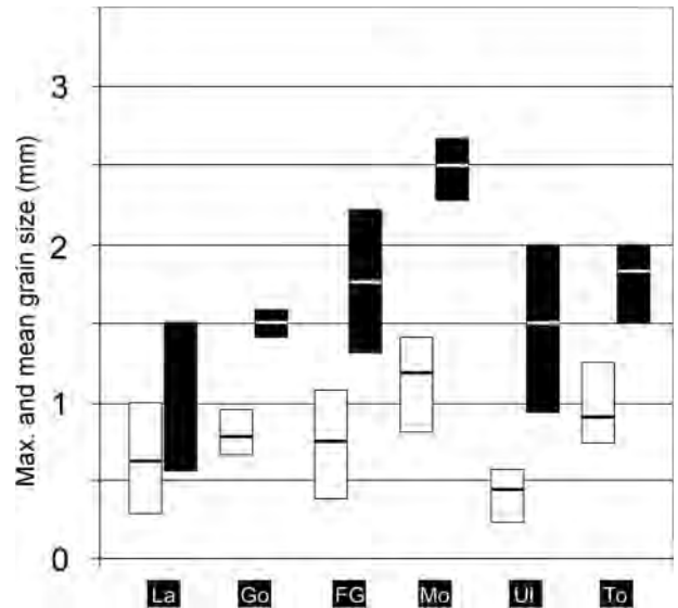
FIGURE 9: Maximum (black bars) and mean (white bars) grain sizes for Laas Marble (La: quarries around Laas; Go: quarries around Gölfan - east of Laas; FG: marble pits between Laas and Gölfan; Mo: quarry at Morter - further east; Ul: Ultental Valley; To: Töll, near Meran).
