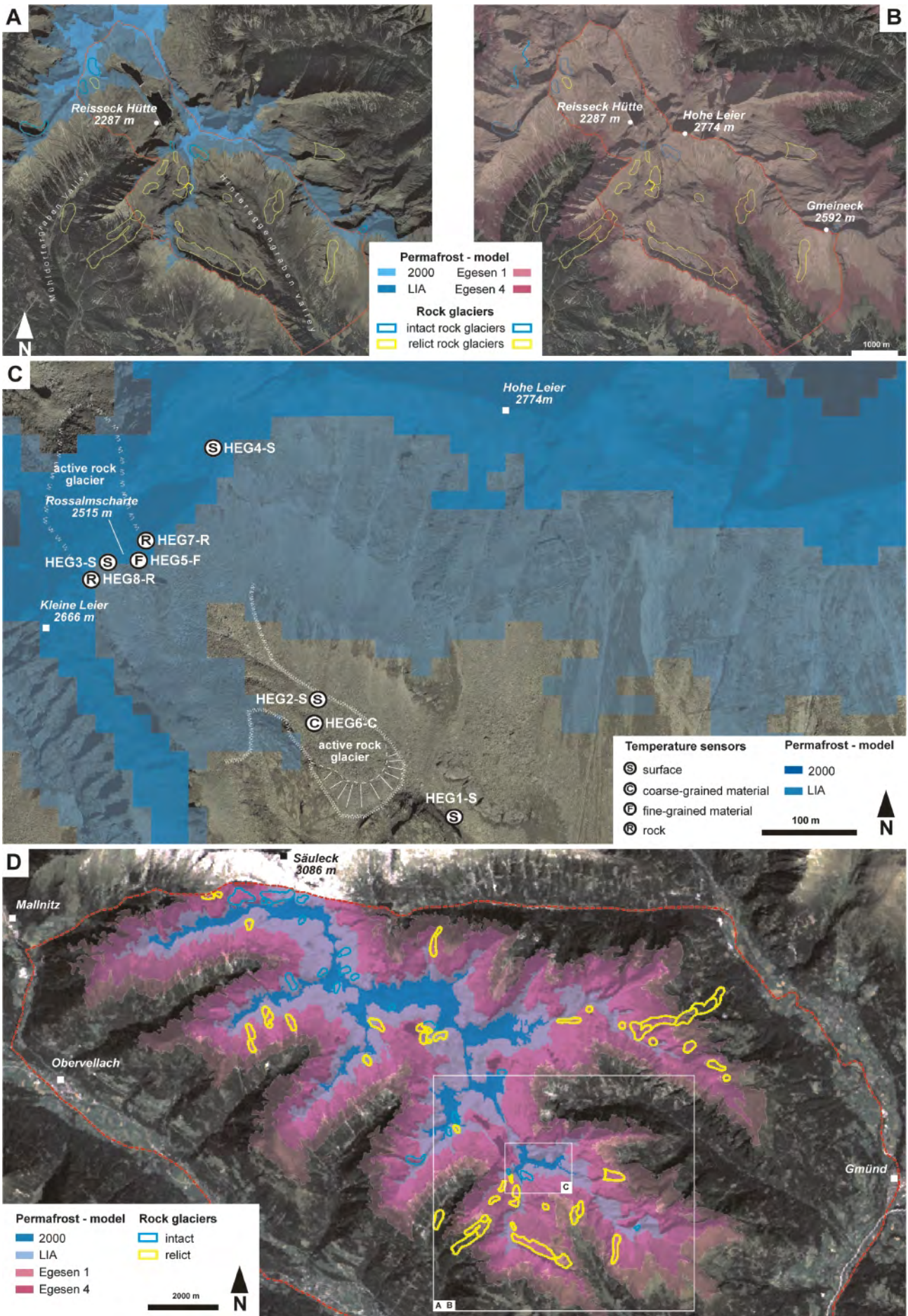
Modelling of potential permafrost distribution during the Younger Dryas, the Little Ice Age and at present in the Reisseck Mountains, Hohe Tauern Range, Austria
