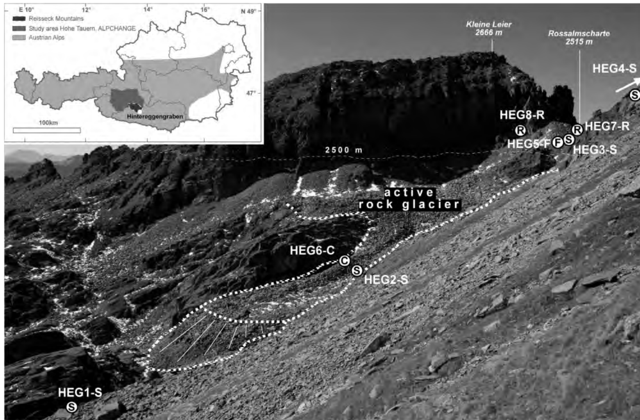
FIGURE 1: The valley head of study area Hintereggen Valley- Hohe Leier (HEG) showing main landforms and temperature sensor sites with respect to surface conditions: S=surface measurement site; C=coarse-debris site, F=fine-grained site; R=rock wall site. Dotted line indicates margin of the rock glacier. Insert maps shows location of the project area of the ALPCHANGE project within Austria, the study region Reisseck Mountains as well as the local study area HEG.
