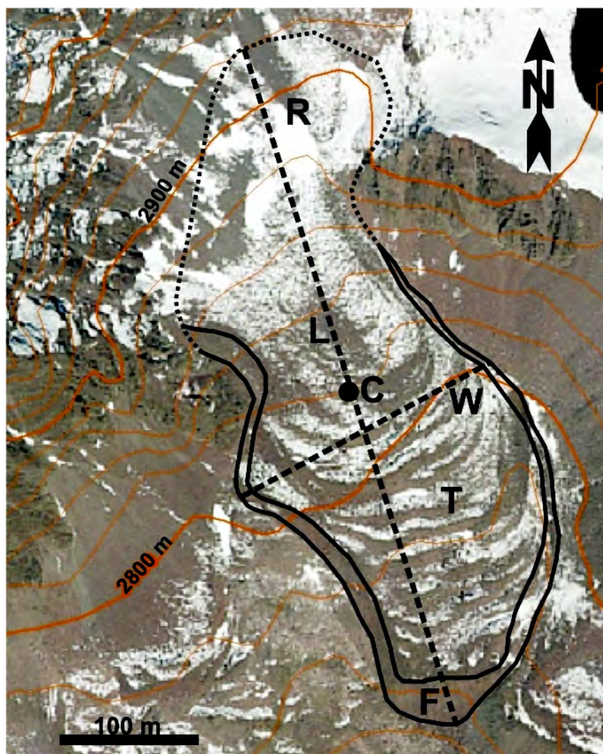
FIGURE 2: Orthophoto of a rock glacier ( www.tirol.gv.at ) with outline and characteristic parameters: R = rooting zone, F = front, T = transverse ridges and furrows, L = length, W = width of the rock glacier. C indicates the point of the coordinates. Due to the steep front which is bare of vegetation and the surface morphology characterized by well developed transverse ridges and furrows this rock glacier is classified as an active rock glacier (OA 304, Schrankar, Stubaier Alpen).
