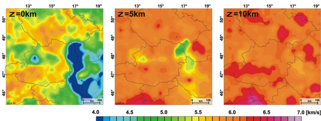
FIGURE 9: Depth slices at ( z = 0 \text{ km} , 5 \text{ km} , and 10 \text{ km} ) through the 3D Vp -velocity model of the upper crust (Behm et al., 2007).
