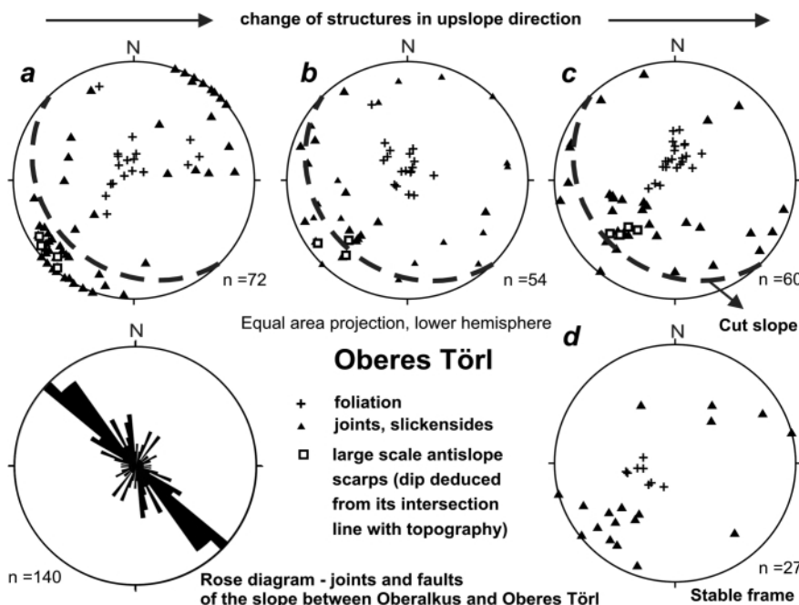
FIGURE 4: Slope of Oberes Törl: Stereo plots of joints, foliation and antislope scarps from the slope segments above Oberalkus (a; approximately 1400 -1900 m a.s.l.), around Unteres Törl (b; approximately 2000-2200 m a.s.l.) and from the uppermost antislope scarps adjoining to the graben structure (c) exposed at the NW flank (see Figs. 1, 2 and 3d). Great circles denote the orientation of the slope with an average gradient of 25^\circ . The plots a-c show an upslope change of these structural elements i.e. concurrent decrease of dip angle of antislope scarps and NE dipping joint system. The orientation of foliation shows a shift from E-SE to S-SW. Downward decreasing rotation of structural elements is also evident by comparison to data from an area 1 km SE of the graben (stereo plot d - "stable frame"; location indicated in Fig. 1) with a subglacially shaped surface and no indication of mass movements. The rose diagram of joints and slickensides displays the dominance of a NW-SE striking joint system parallel to the Isel fault over those with a N-S and NNE-SSW trend.
