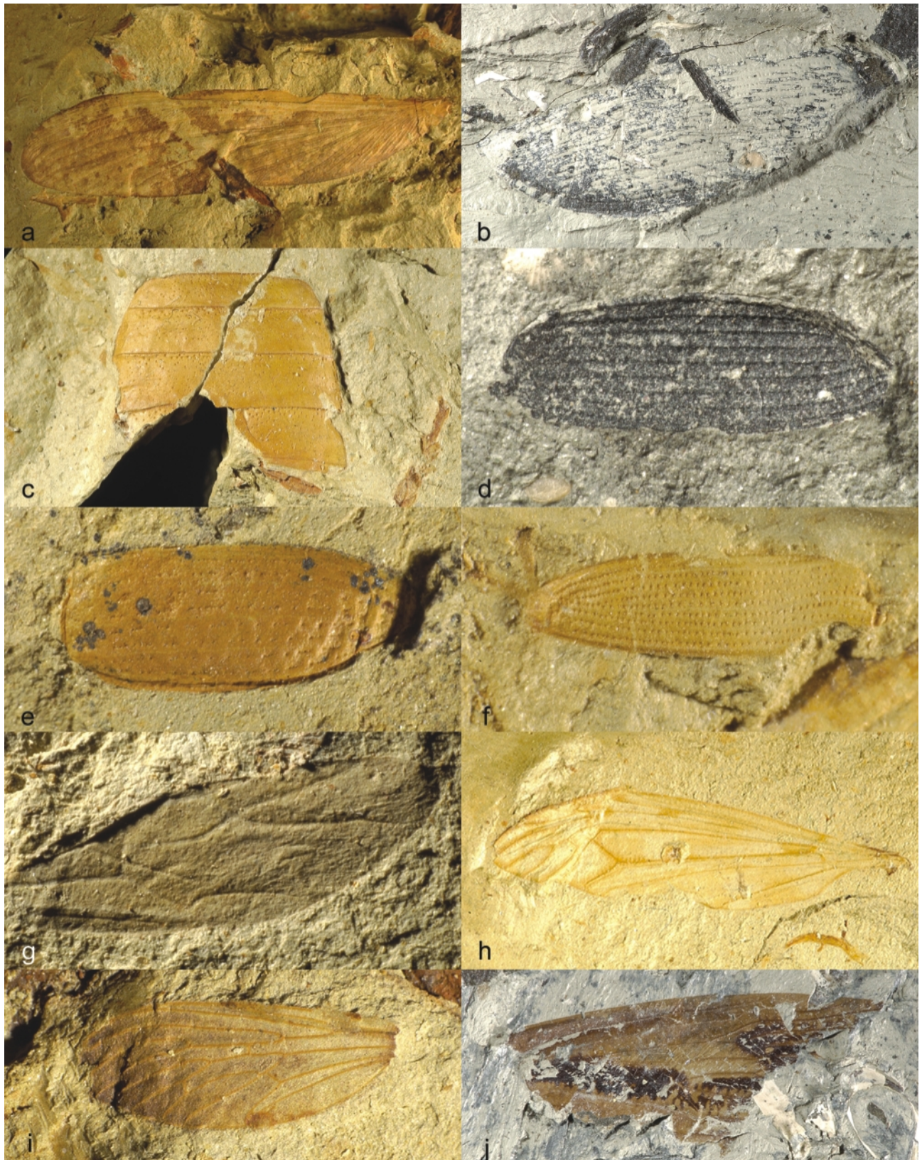
FIGURE 3: Representative diversity of Pannonian-age insects from Styria. (a) A new genus and species of giant termite (Isoptera), Paldau, LMJ 204.149 (wing length 33.5 mm). (b) Elytron of an indeterminable family of beetles (Coleoptera), Mataschen, LMJ 204.157 (elytron length 19.9 mm). (c) Abdominal sterna of an indeterminable beetle (Coleoptera), Paldau, LMJ 204.153 (length of abdomen 9.3 mm). (d) Elytron of a ground beetle, perhaps near Pterostichus (Coleoptera: Carabidae), Mataschen, LMJ 201.116 (elytron length 7.7 mm; specimen originally reported by Gross, 2004a). (e) Elytron of a ground beetle (Coleoptera: Carabidae), Paldau, LMJ 204.154 (elytron length 7.5 mm). (f) Elytron of a possible donacine leaf beetle (Coleoptera: Chrysomelidae), Münzengraben, LMJ 204.156 (elytron length 7.1 mm). (g) A formicine ant forewing (Hymenoptera: Formicidae), Paldau, LMJ 204.150 (wing length 14.3 mm). (h) A new species of crane fly, genus Tipula (Diptera: Tipulidae), Paldau, LMJ 204.151 (wing length 18.7 mm). (i) A generalized brachyceran fly wing, perhaps of the snipe fly family Rhagionidae (Diptera: Brachycera), Paldau, LMJ 204.155 (wing length 6.7 mm). (j) A large caddisfly perhaps allied to the genus Agrypnia (Trichoptera: Phrygaenidae), Mataschen, LMJ 204.158 (wing length 20.1 mm).
