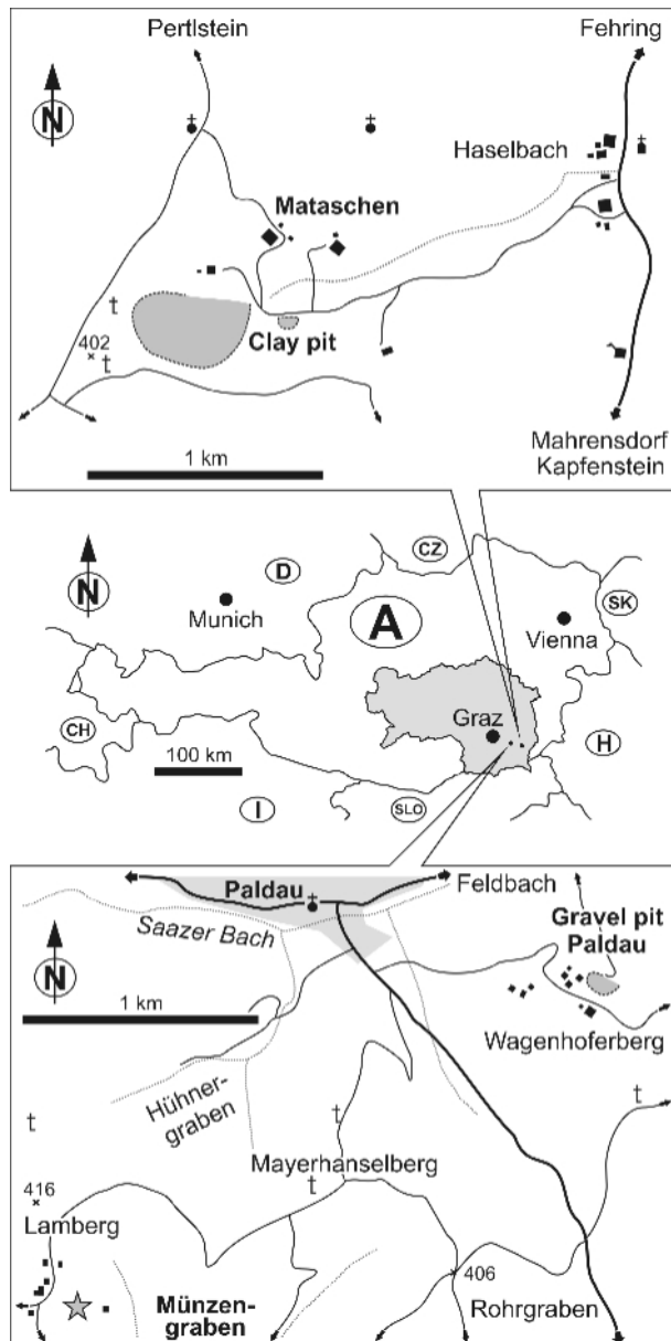
FIGURE 1: Geographic setting of insect-bearing Pannonian localities in the Styrian Neogene Basin (Mataschen, 46°54'15"N, 15°57'16"E; Paldau 46°56'17"N, 15°48'37"E, Münzengraben 46°55'39"N, 15°47'09"E).
