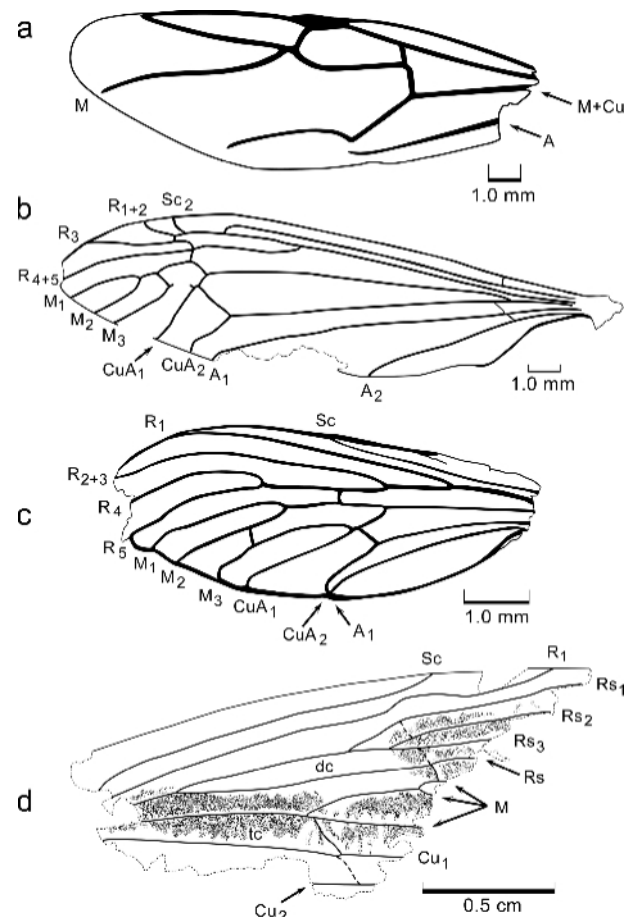
FIGURE 4: Forewing venations of four insects from the Pannonian of Styria. (a) A winged ant (Formicidae) likely of the Formicinae (LMJ 204.150). (b) A new species of crane fly (Tipulidae: Tipula sp.) (LMJ 204.151). (c) A generalized brachyceran fly, perhaps a snipe fly (Diptera: Rhagionidae?) (LMJ 204.155). (d) A phrygaenid caddisfly, perhaps near the genus Agrypnia (Trichoptera: Phrygaenidae) (LMJ 204.158) (dc = discoidal cell; tc = thyridium cell).
