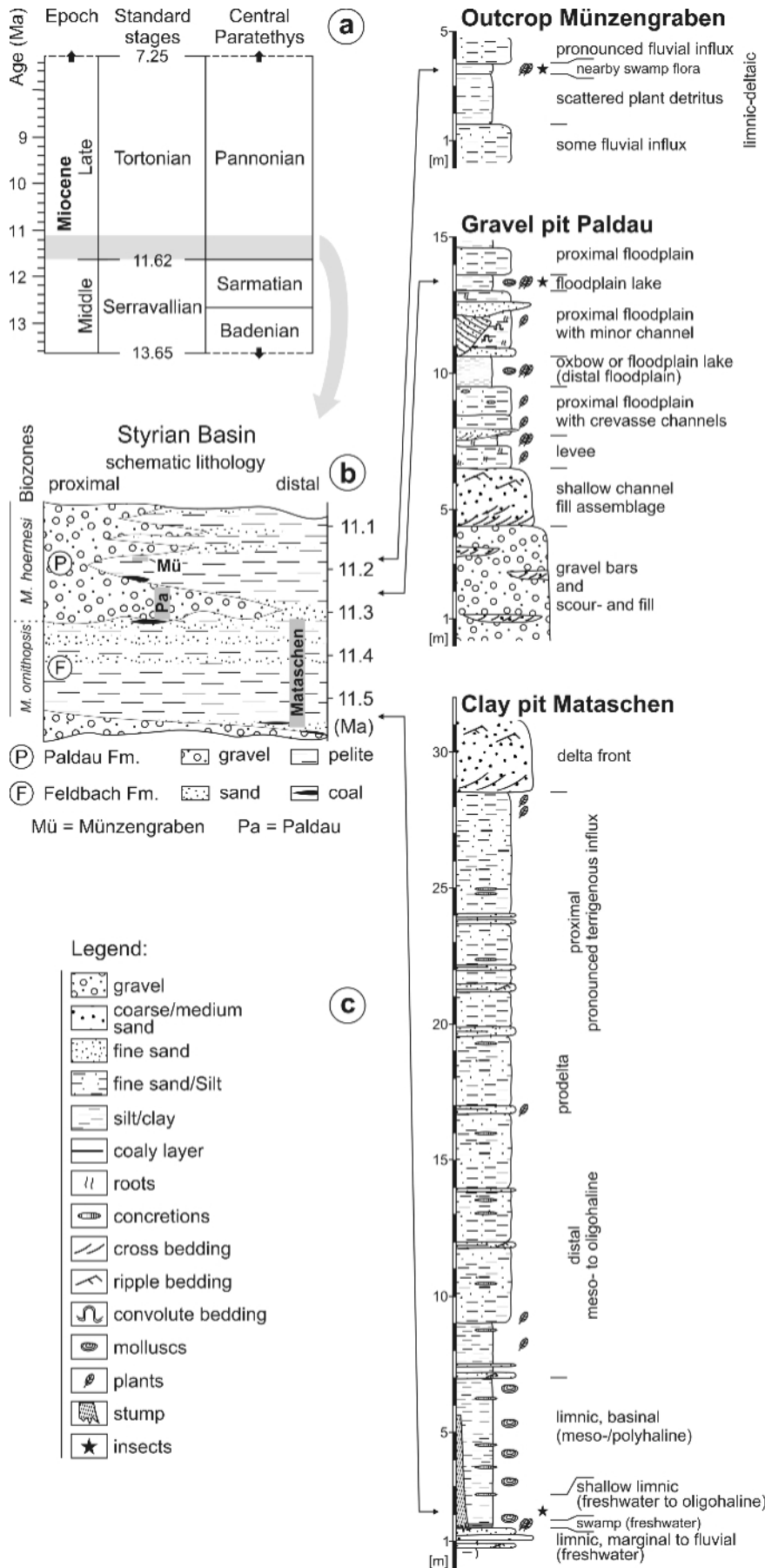
FIGURE 2: Stratigraphy, profiles, and facies interpretation of the Pannonian insect localities of Styria. (a) Correlation of Standard and Central Paratethys stages. (b) Litho- and biostratigraphical scheme of Lower Pannonian sediments in the Styrian Basin. (c) Profiles and proposed sedimentary environment.
