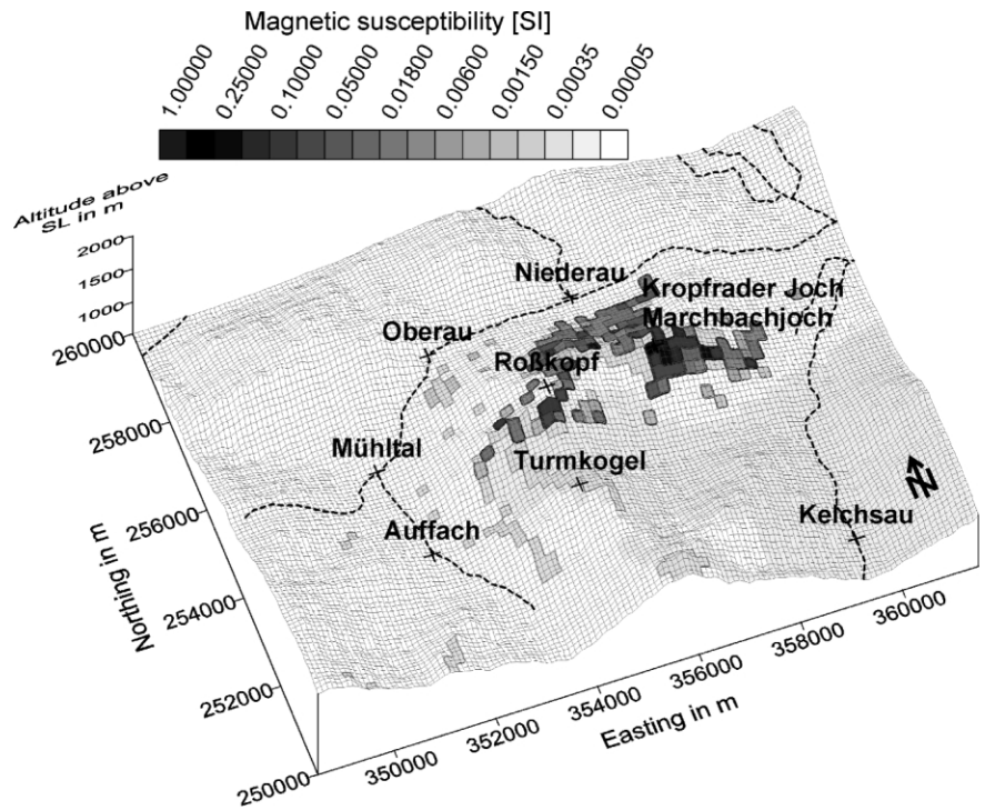
FIGURE 17: Model area Würgl: modelled magnetic susceptibility at the surface. (Roads and some geographic points are shown, coordinate system is Austrian BMN zones M31).
