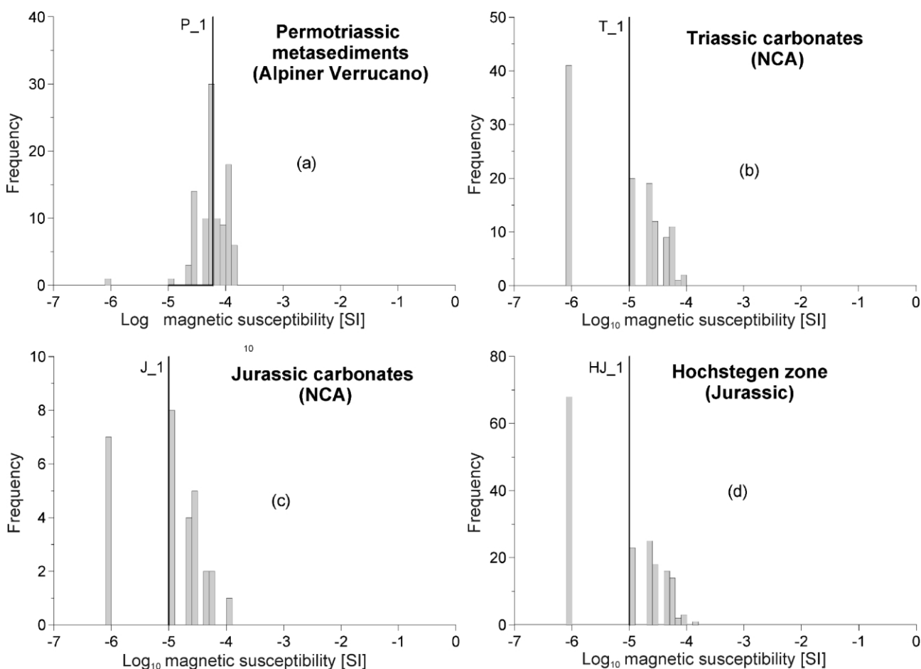
FIGURE 4: Distribution of the magnetic susceptibility of Permotriassic, Triassic and Jurassic rocks. (a) siliclastic "Alpine Verrucano", NCA, (b) Triassic carbonates of the NCA, calcitic and dolomitic marbles of the Seidwinkeltrias and dolomitic marbles of the Krimmler Triassic rocks (c) Jurassic (mainly Liassic) carbonates of the NCA, (d) Jurassic Hochstegen marble of the Venediger nappe (Mesozoic cover of the Sub-Penninic Ahorn core).
