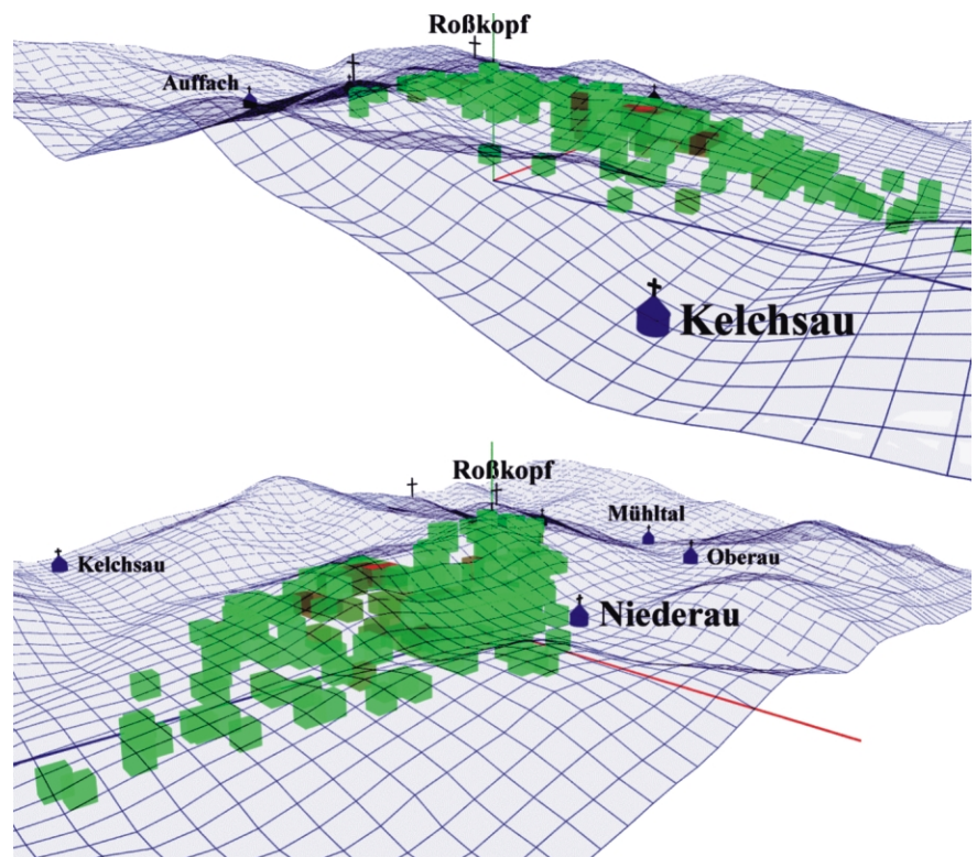
FIGURE 18: 3D model of the magnetic anomalies in Würgl area. The cubes of the model (200 x 200 x 200 m) are shown as green cubes. The thin red bar in the center of the figure points to the north, the blue bar to the east.
